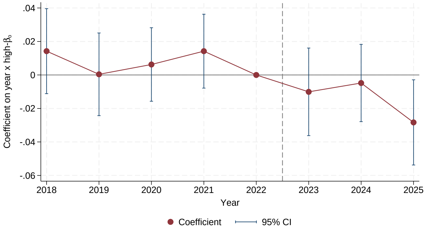
Log Wage: binarized treatment, full sample
