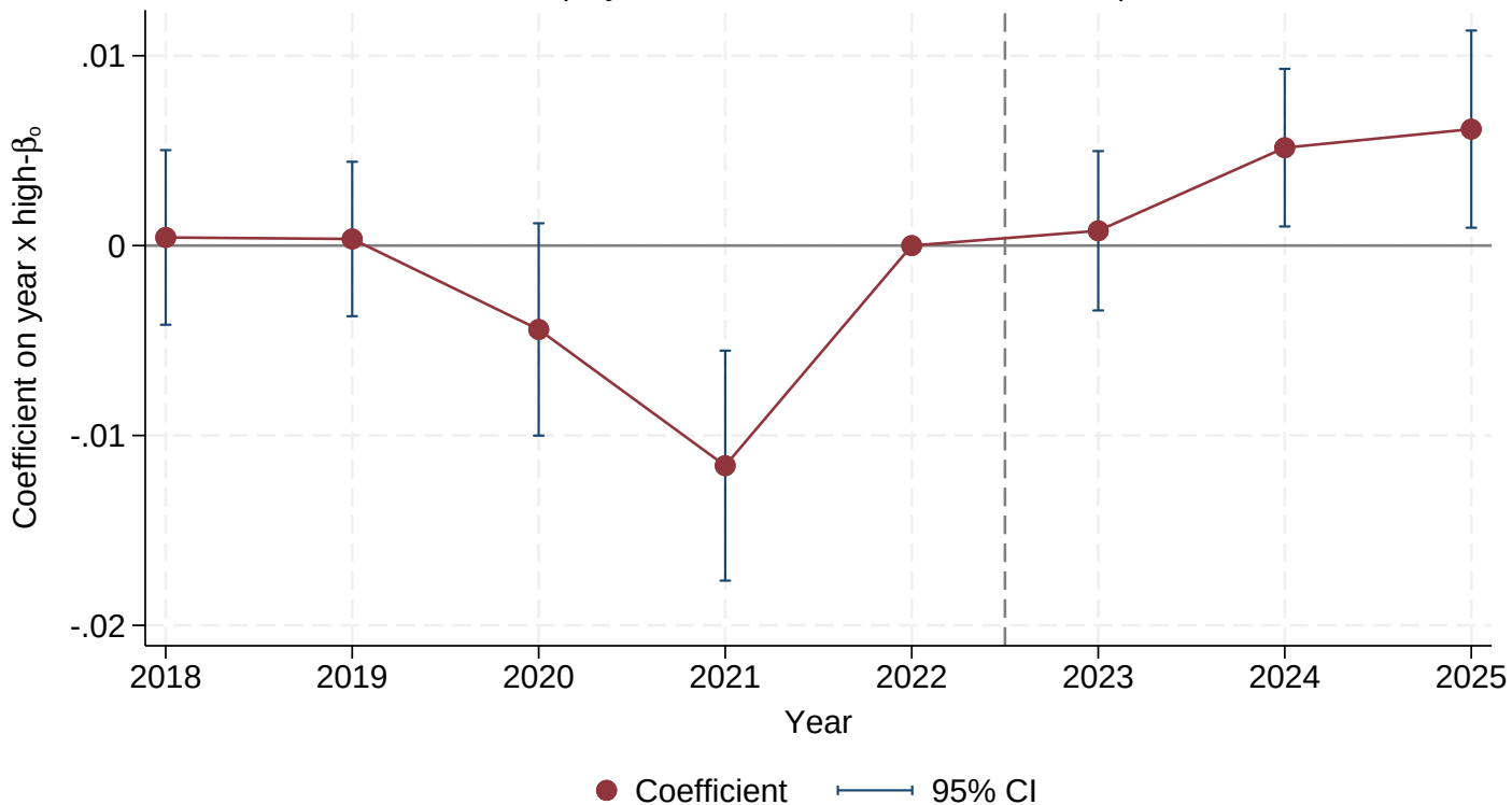
Unemployment: binarized treatment, full sample
