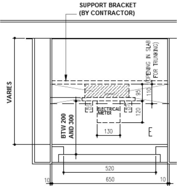
TYPICAL DETAIL OF ELECTRICAL RISER / METER DUCT SCALE: N.T.S.
