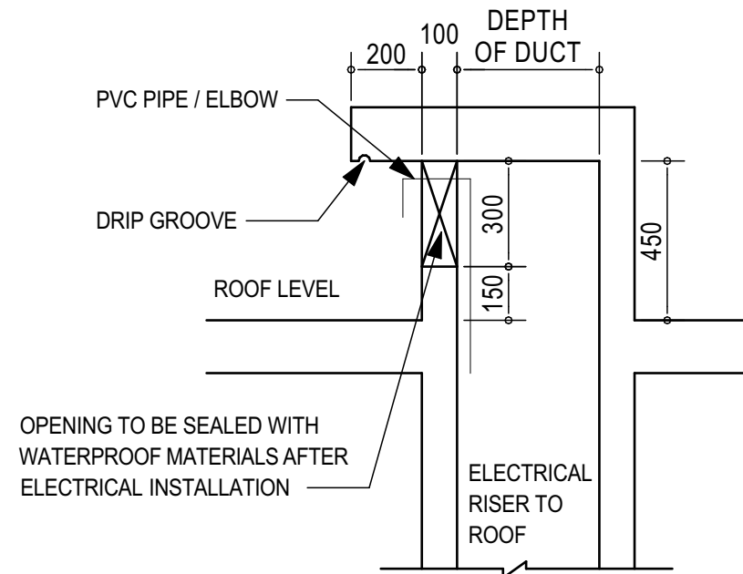
TYPICAL DETAIL OF DOG HOUSE OF ELECTRICAL CABLES ON ROOF SCALE: N.T.S.
