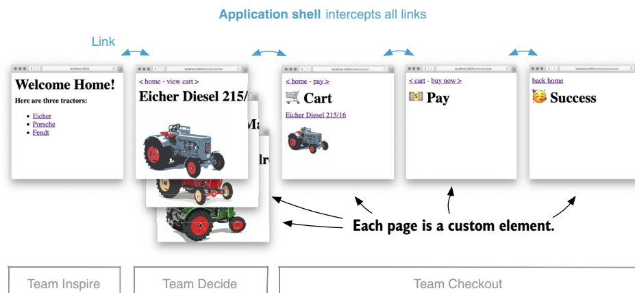
Figure 7.5 The pages in the example project are connected via links. The application shell intercepts these links and performs a soft navigation to the requested page. Teams expose their pages as Custom Elements. On navigation, the app shell replaces the existing page component with the new one.
