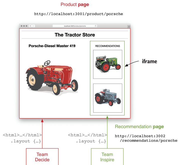
Figure 2.6 Integrating the recommendation page into the product page via iframe. These pages don't share anything. Both are standalone HTML documents with their own styling.
