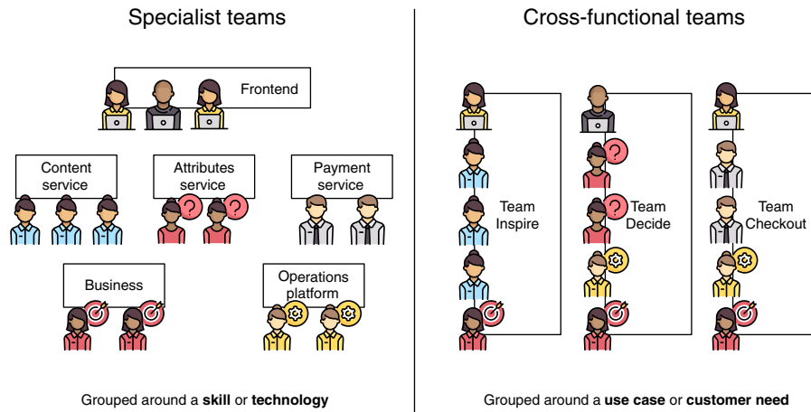
Figure 1.3 Team structure of a microservice-style architecture on the left compared with micro frontends teams on the right. Here the teams are formed around a customer need and not based on technologies like frontend and backend.
