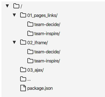
Figure 2.2 The directory structure of the example code bundle. The main directory (shown as /) contains a sub-folder for each example project. The top-level package.json file contains the run commands for all examples.
