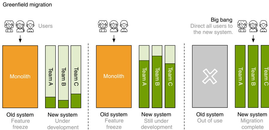
Figure 14.4 We set up our new team structure and system architecture beside the existing monolith (left). The new and old systems don't share anything. During the development phase, all incoming traffic still arrives at the monolith (middle). When the teams finish building the new system, we direct the incoming traffic to the new system, and the monolith is out of use (right).
