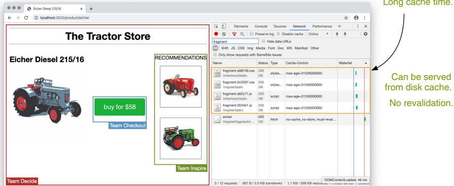
Figure 10.3 Shows the browser's Network tab with the fragment assets required for this page. The HTML directly links to the fingerprinted files from the other teams. The assets are cacheable for a long time.
