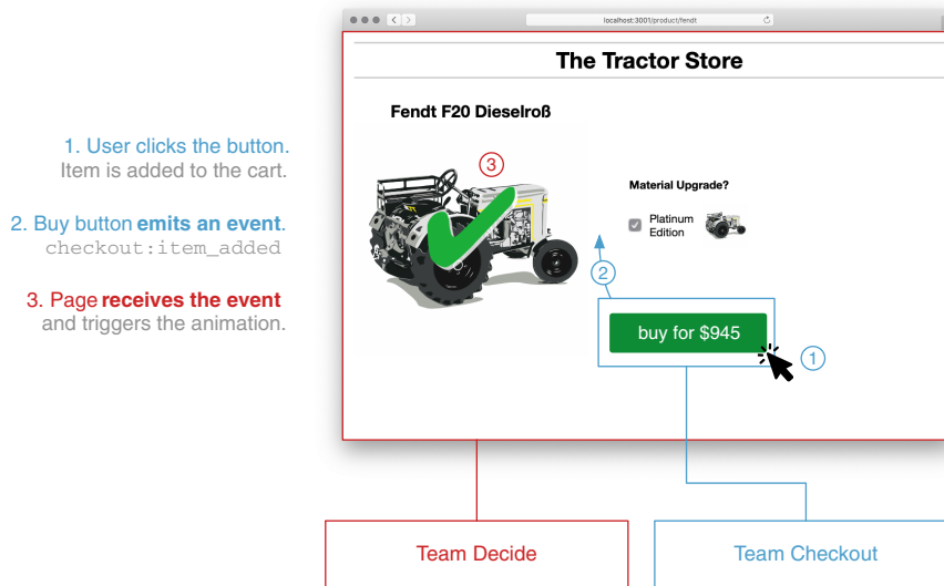
Figure 6.5 Team Checkout's Buy button emits an event when the user adds an item to the cart. Team Decide reacts to this event and triggers an animation on the main product image.
