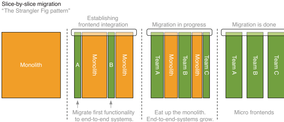
Figure 14.2 Migrating a monolithic application (left) to a three-team micro frontends architecture (right). In this diagram, we create three new applications (Team A-C), which take over functionality from the monolith step by step until the monolith has vanished (middle). Like in the previous example, we start with establishing the required frontend integration mechanism that handles the routing and composition of the different applications.
