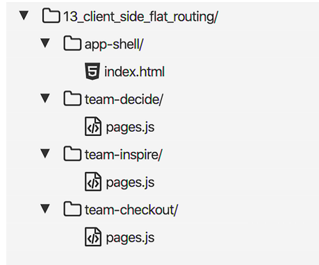
Figure 7.4 The app shell’s code is located beside the team’s code. It provides a shared HTML document. The teams just deliver page components via JavaScript.
