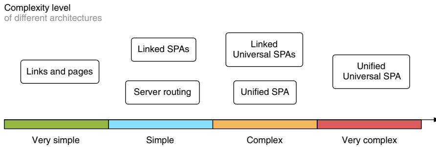
Figure 9.3 Micro frontend architectures sorted by complexity. The links and pages approach is the simplest one to build and run. The complexity rises as you move to more sophisticated architectures. The Unified Universal SPA approach requires a lot of development skills to get it right. You also need shared infrastructure and code to make it happen.
