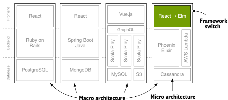
Figure 1.11 Teams can decide about their internal architecture (micro architecture) on their own as long as they stay in the boundaries of the agreed upon macro architecture.
