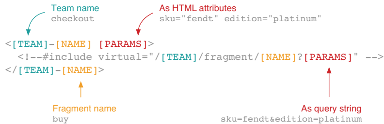
Figure 8.5 This schema shows how you could generate the universal integration markup in a standardized way. When offering or integrating a fragment, teams need to know three properties: the name of the team that owns it, the name of the micro frontend itself, and the parameters it takes.
