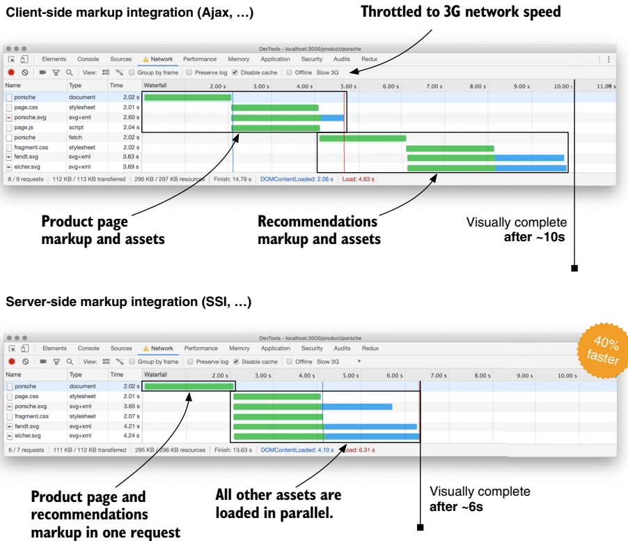
Figure 4.3 Page-load speed for the product page with client-side and server-side composition. Server-side integration optimizes the critical paths.
