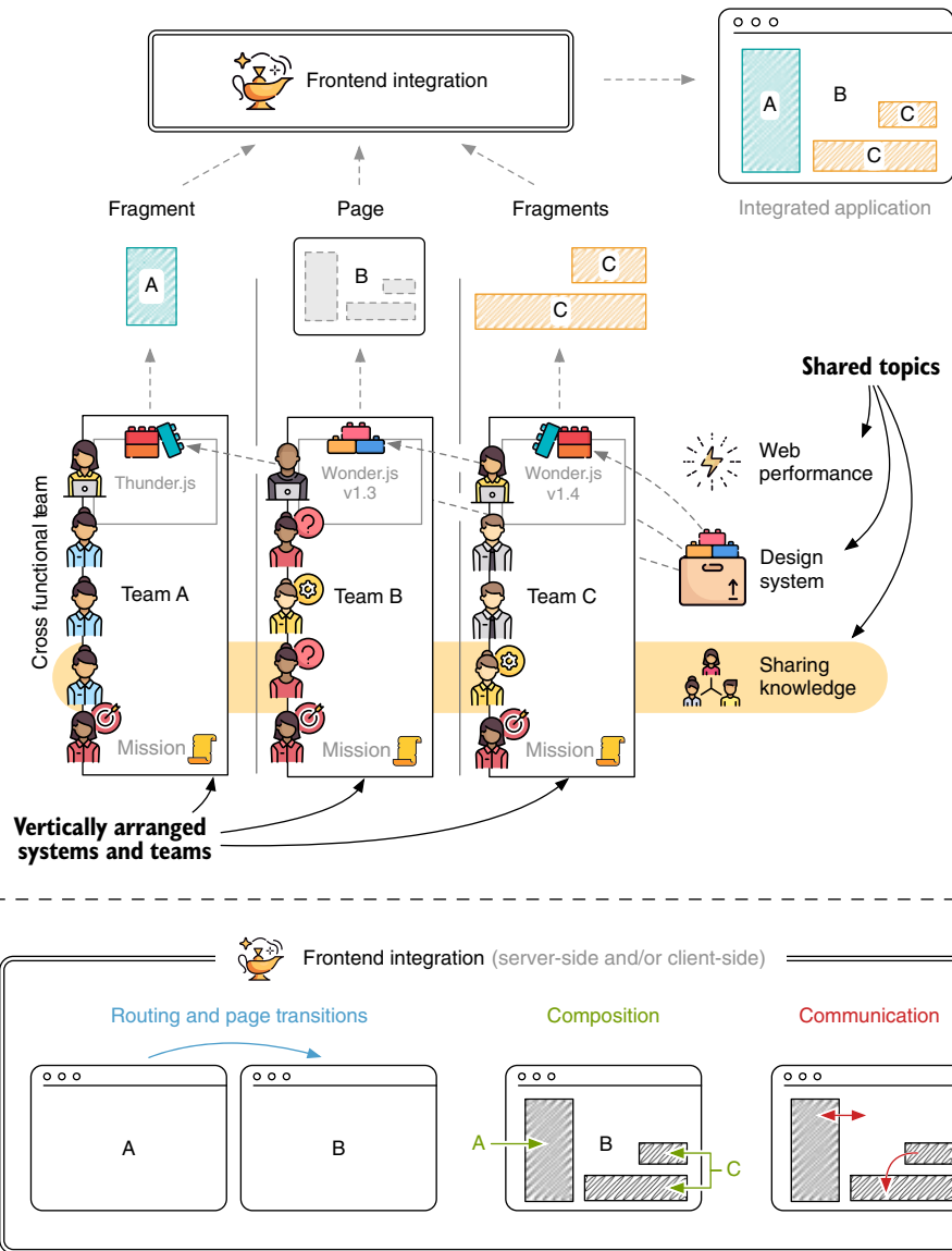
Figure 1.1 Here is the big picture overview of the micro frontends approach. The vertically arranged teams at the bottom are the core of this architecture. They each produce features in the form of pages or fragments. You can use techniques like SSI or Web Components to integrate them into an assembled page that reaches the customer.
