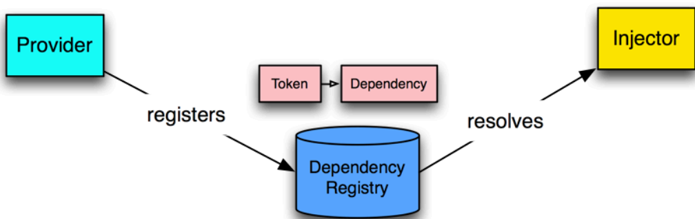
Dependency Injection
