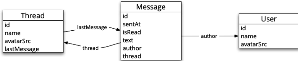
Chat Models
