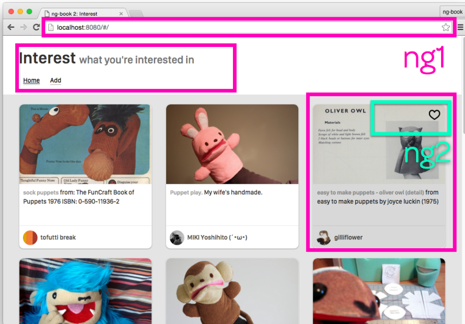
Homepage ng1 and ng2 Components
