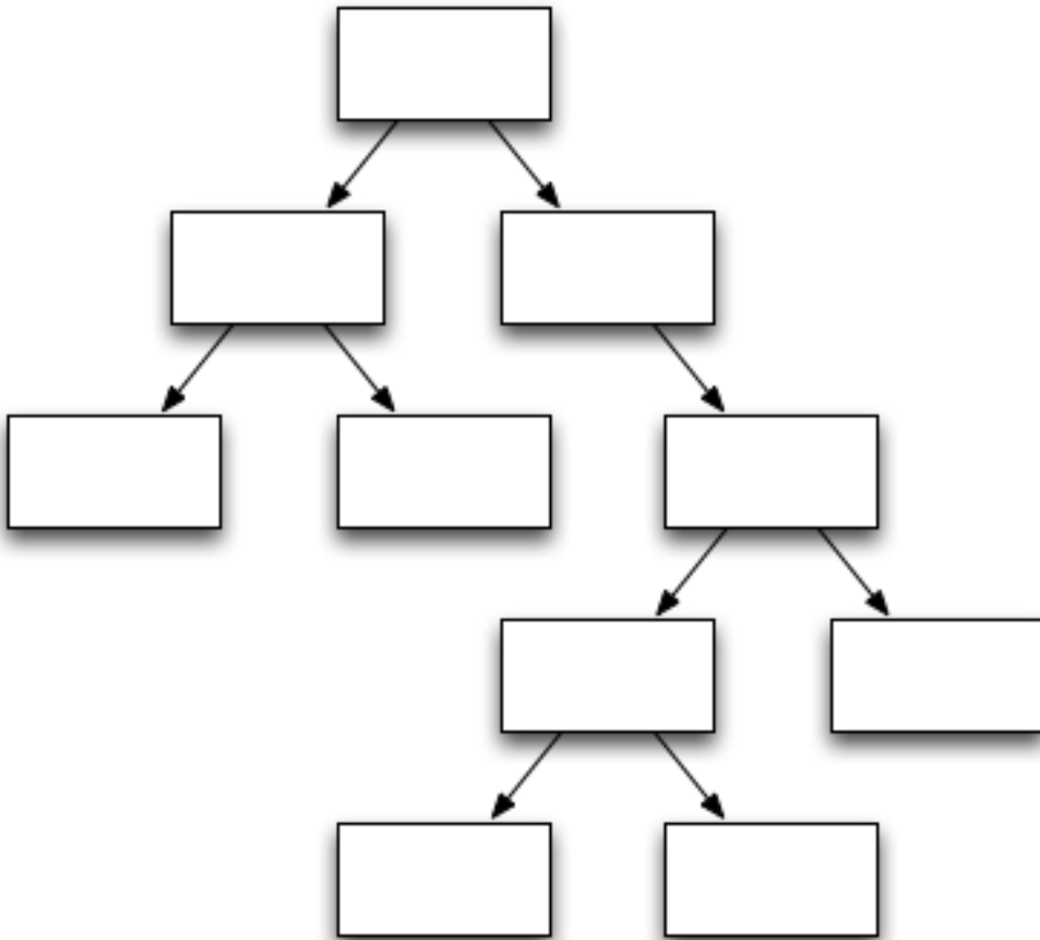
Component tree
