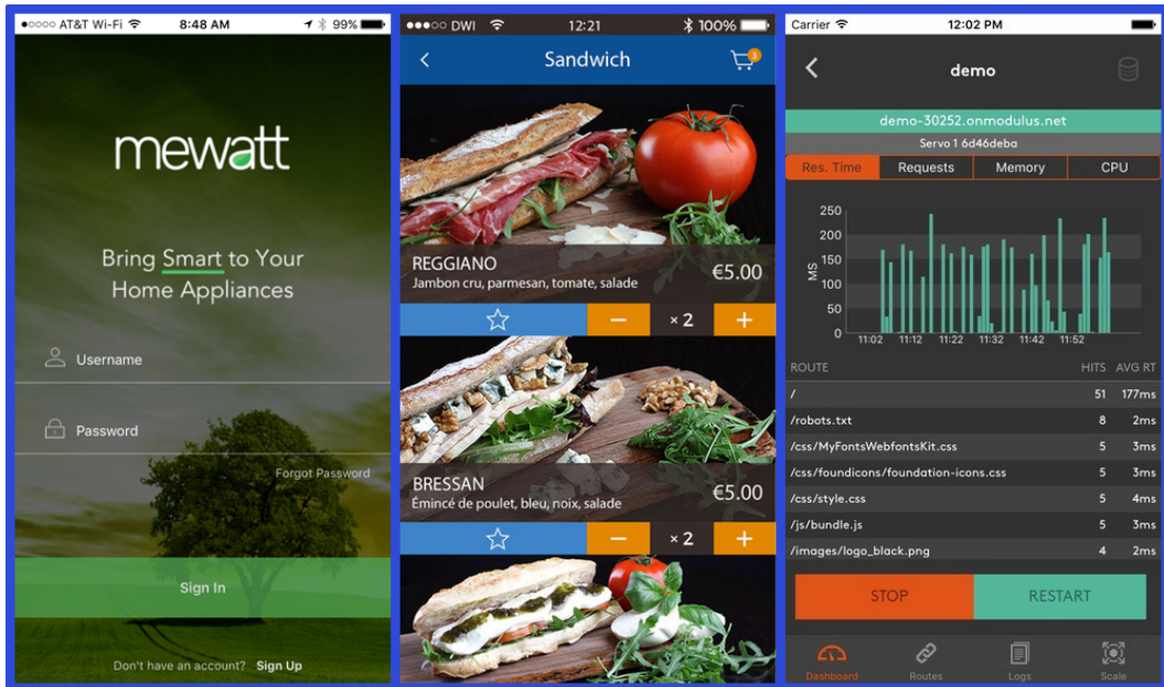
NativeScript Showcase
