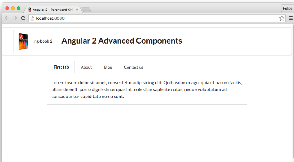
Tabset application
