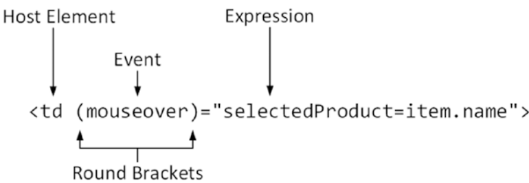
Figure 14-3. The anatomy of an event binding
