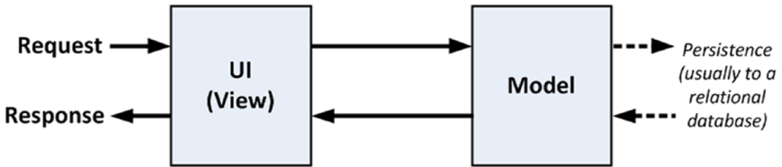
Figure 3-3. The model-view pattern
