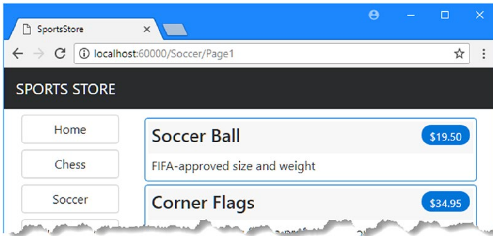
Figure 9-3. Generating category links with a view component
