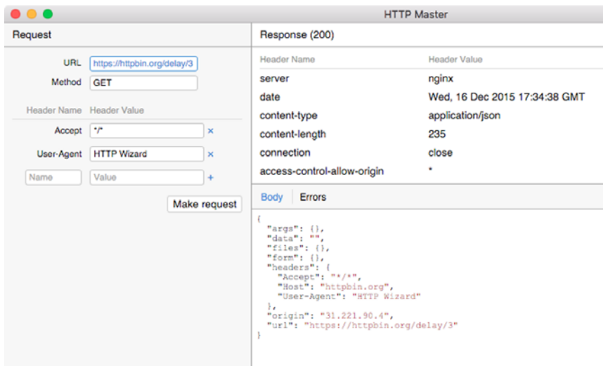
Figure 12.4 The HTTP Master Electron application
