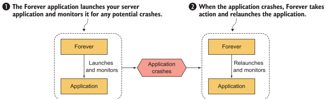
Figure 10.1 The Forever tool helps you keep your application running, even if it crashes.
