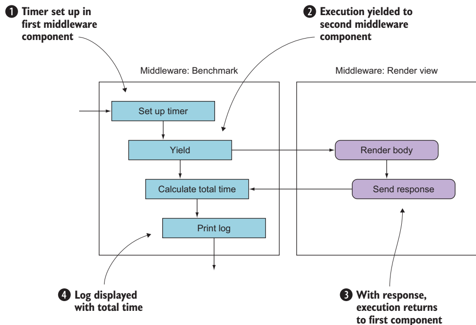
Figure 5.1 Koa middleware execution order
