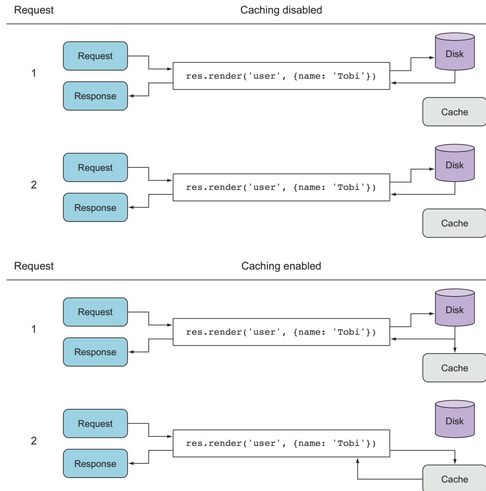
Figure 6.9 The view cache setting
