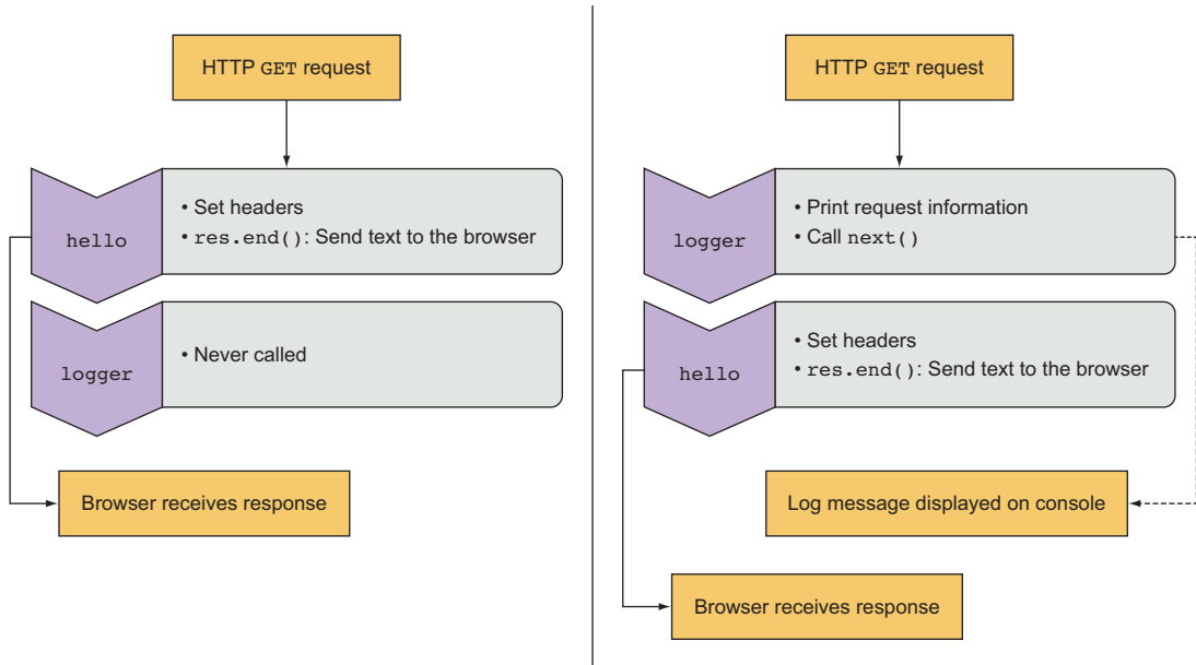
Figure 6.2 Middleware ordering is important.
