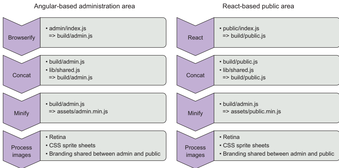
Figure 4.1 Two build processes that share functionality
