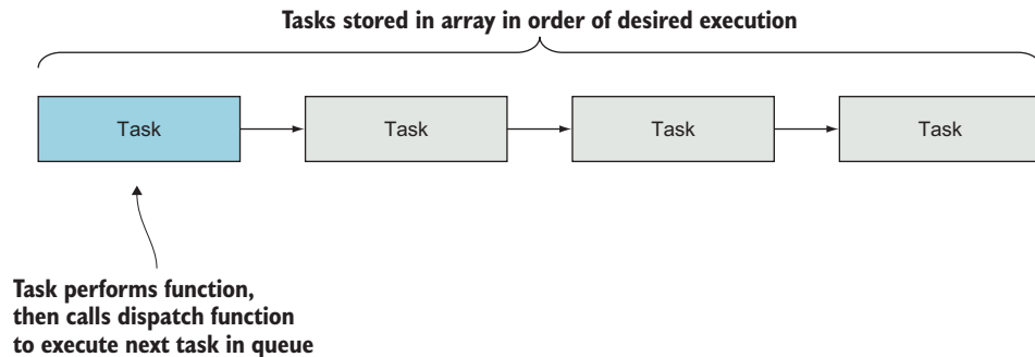
Figure 2.11 How serial flow control works
