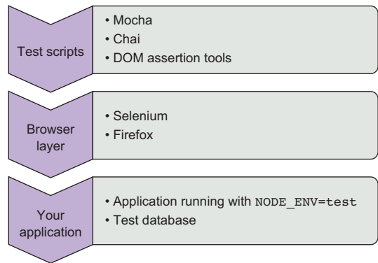
Figure 9.6 Testing with browser automation
