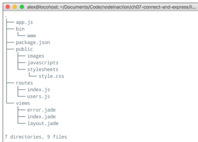
Figure 6.4 Default application skeleton structure using EJS templates
