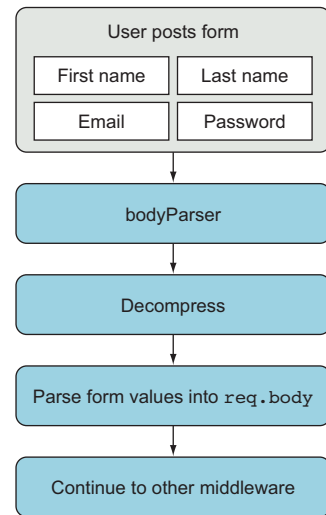
Figure C.1 How a form is processed by body-parser
