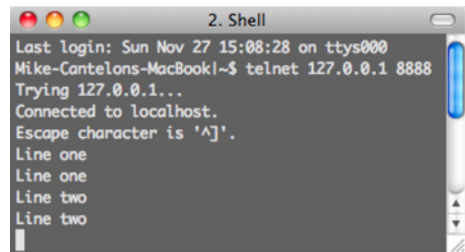
Figure 2.9 An echo server repeating the data sent to it
