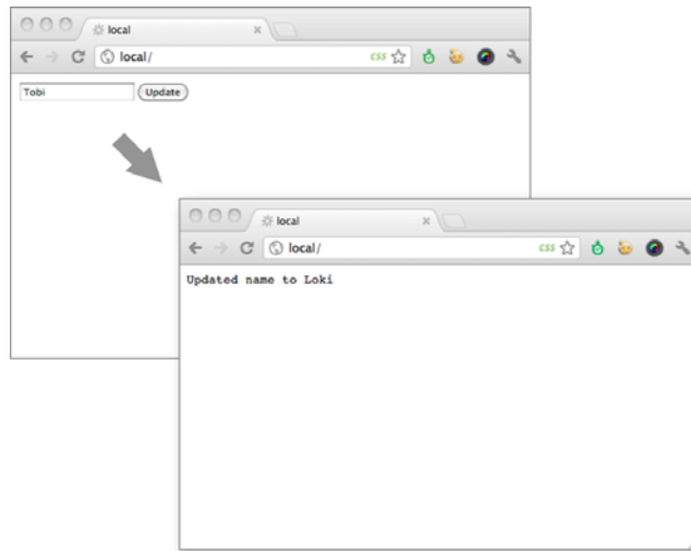
Figure C.3 Using method-override to simulate a PUT request to update a form in the browser
