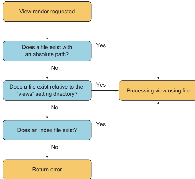
Figure 6.10 Express view lookup process
