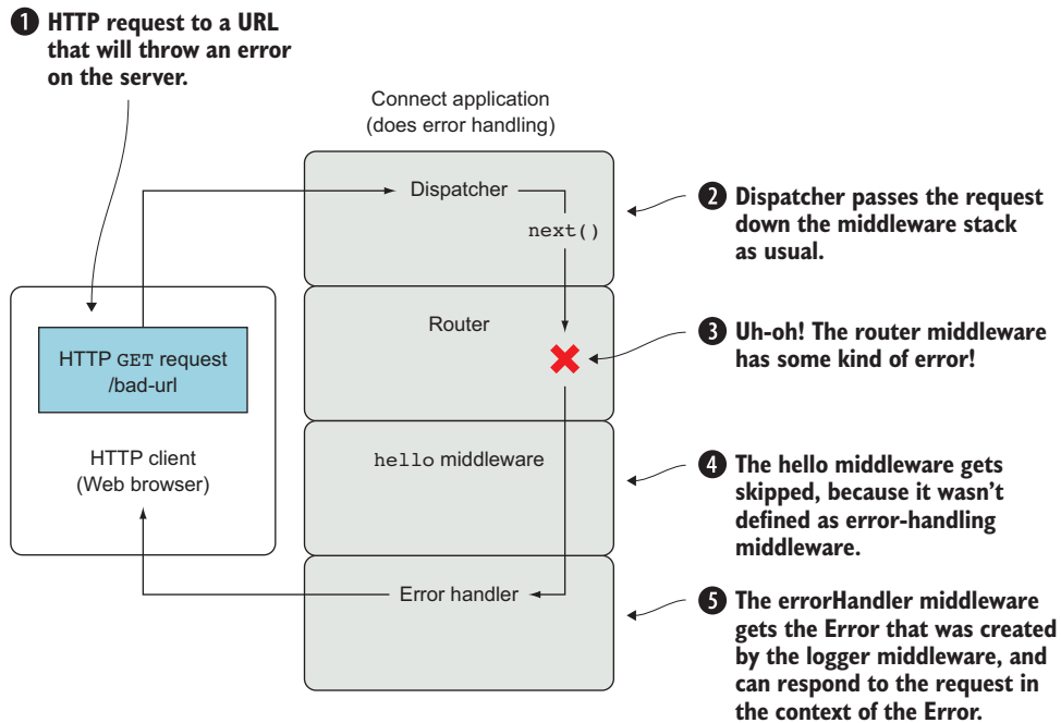
Figure 6.3 The life cycle of an HTTP request causing an error in a Connect server
