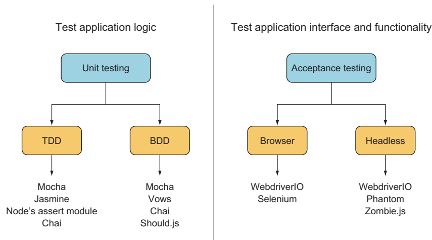
Figure 9.1 Test framework overview
