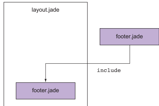
Figure 7.3 Pug's include mechanism provides a simple way to include the contents of one template in another template during rendering.
