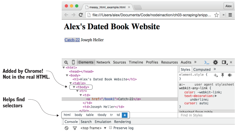
Figure B.4 Viewing HTML in Chrome
