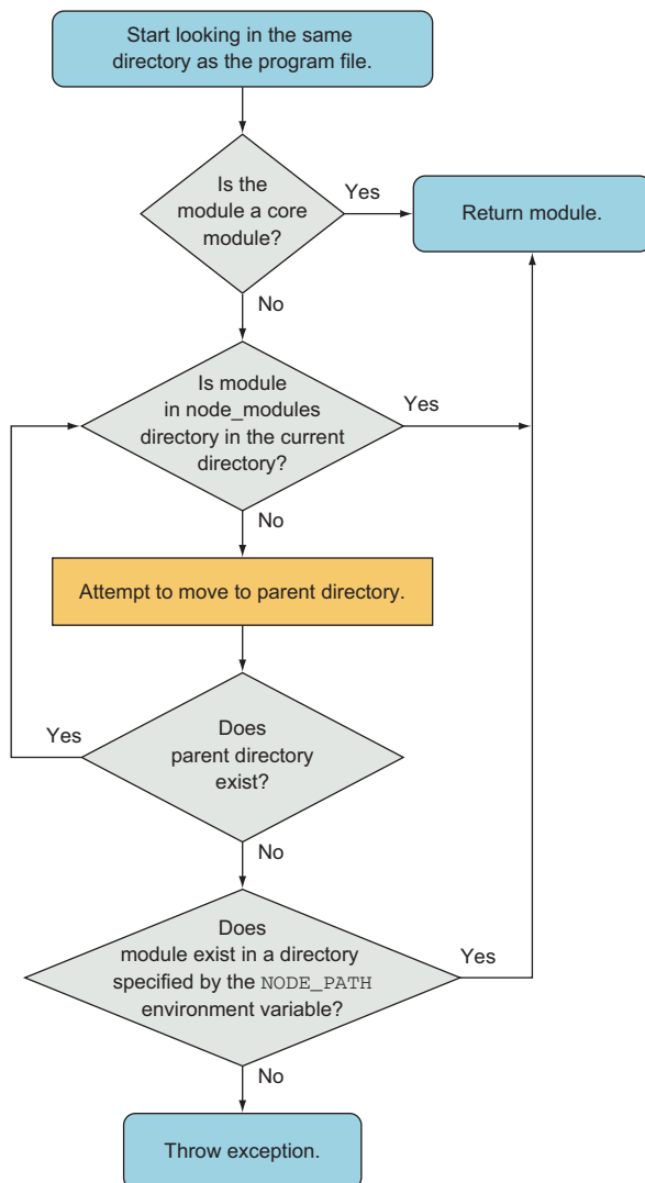
Figure 2.5 Steps to finding a module
