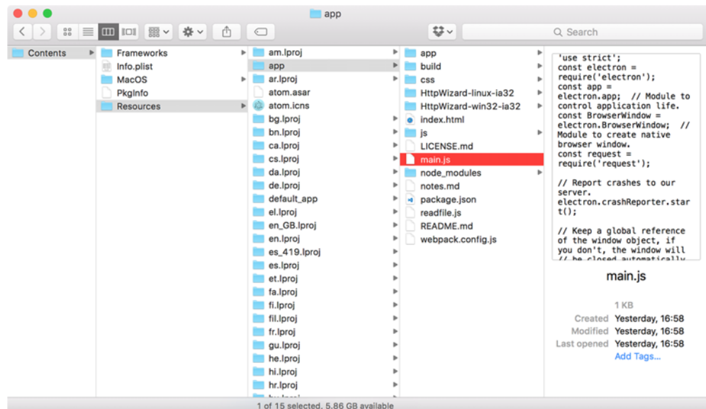
Figure 12.6 A typical Electron application bundle's contents
