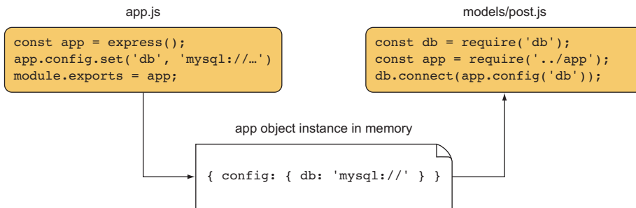
Figure 2.7 Shared app object in a web app
