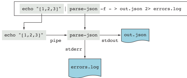
Figure 11.2 Combining pipes and output streams
