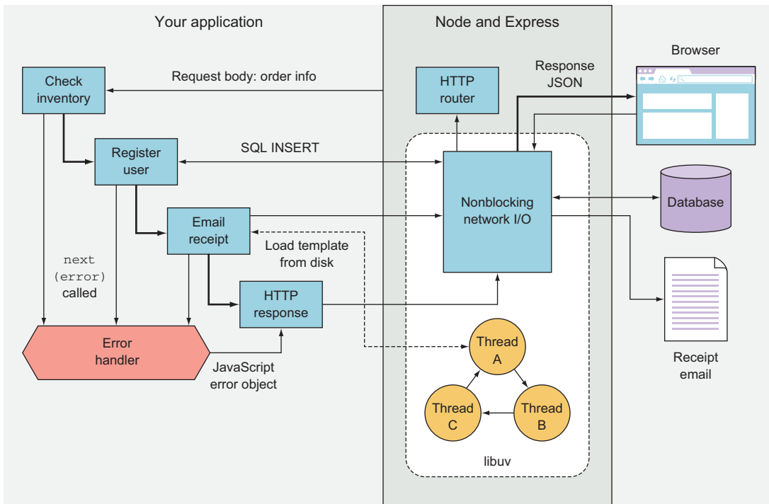
Figure 1.1 Asynchronous and nonblocking components in a Node application
