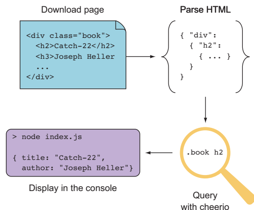
Figure B.3 Scraping with cheerio
