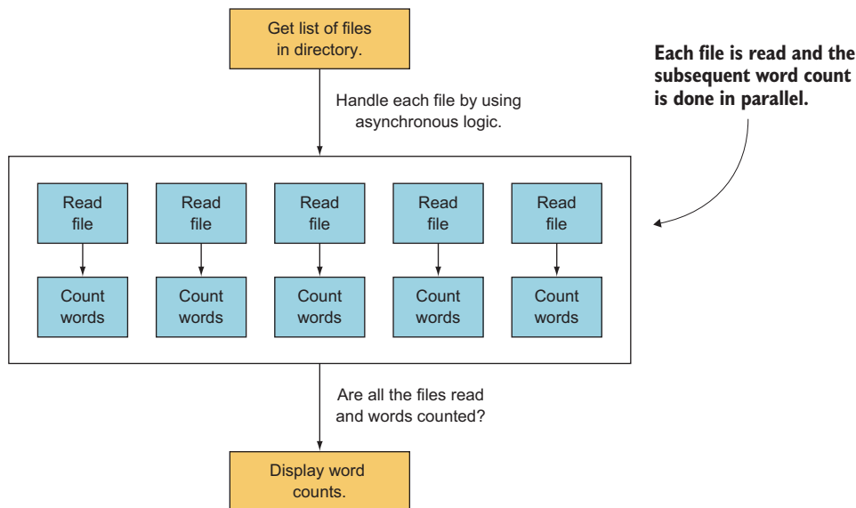
Figure 2.12 Using parallel flow control to implement a frequency count of word use in numerous files
