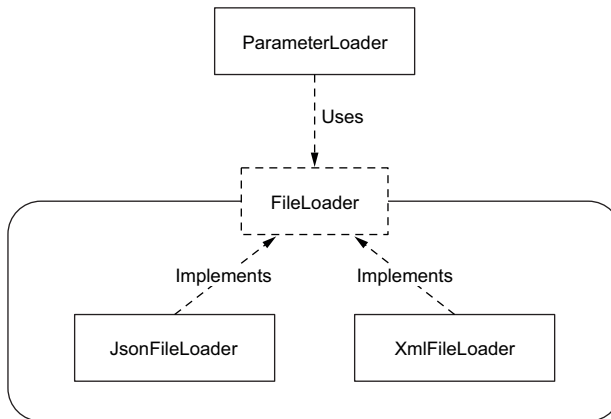
Figure 9.1 As long as the FileLoader dependency of ParameterLoader follows the contract defined by the interface, it doesn't matter what goes on behind the scenes of the real FileLoader that gets injected.
