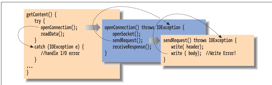
Figure 6-3. Exception propagation
