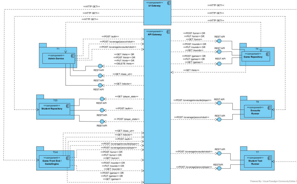
Figure 10: Component Diagram
