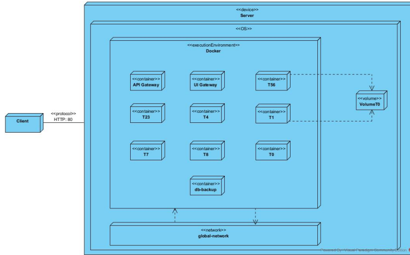
Figure 16: Deploy Diagram
