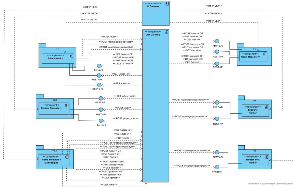
Figure 11: Component Diagram
