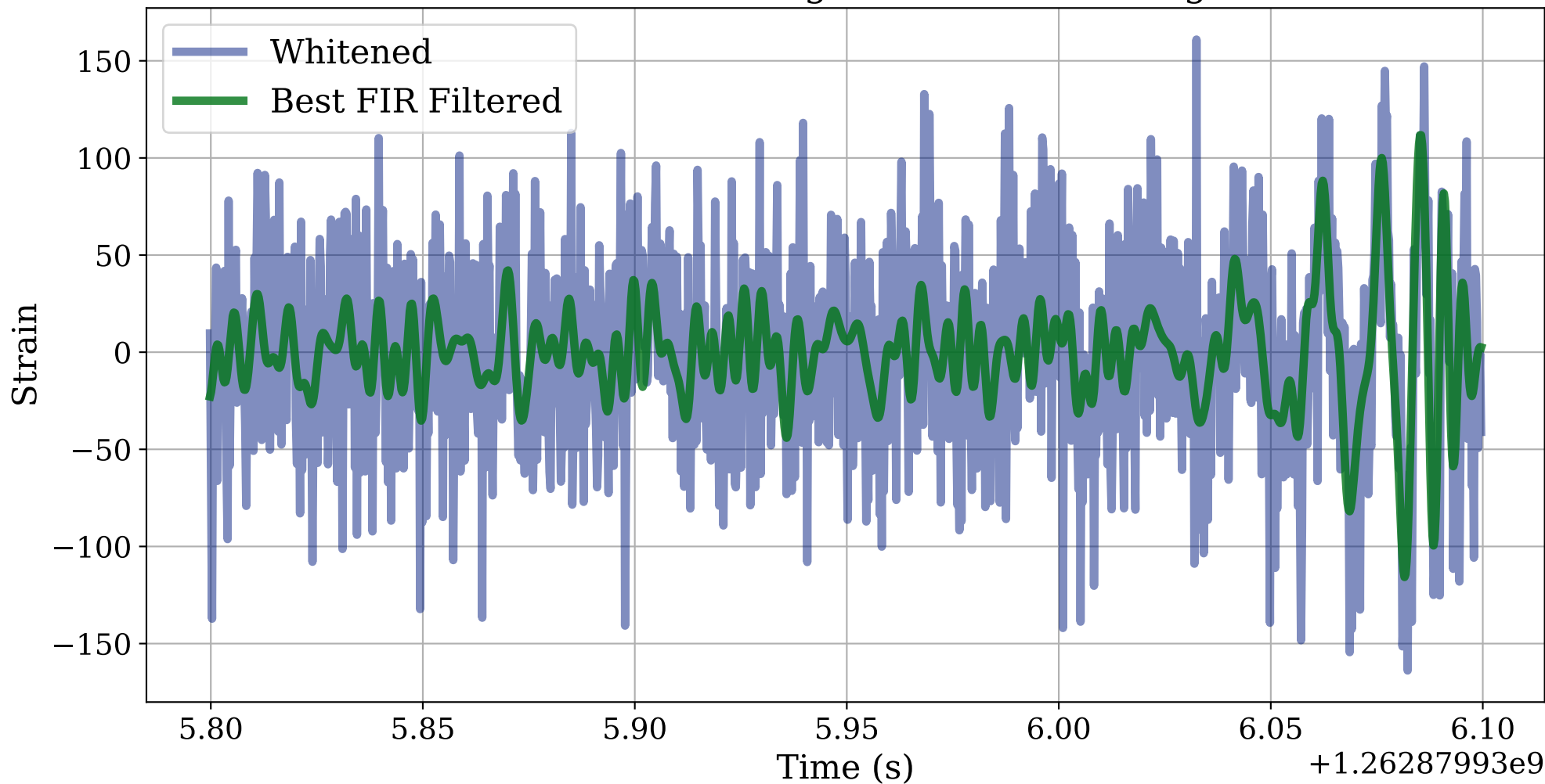
Best FIR Filtered Signal vs Whitened Signal
