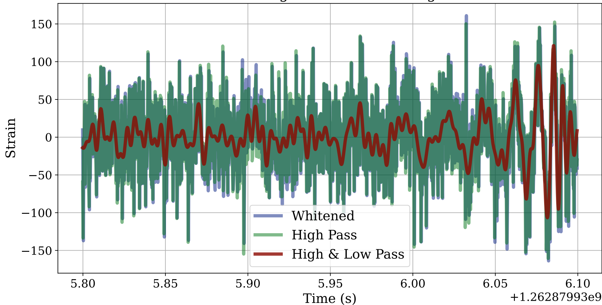
Filtered Signal vs Whitened Signal
