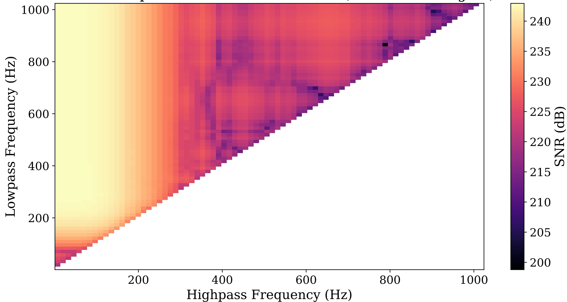
SNR Heatmap for FIR Filter Parameters (Unwhitened Signal)
