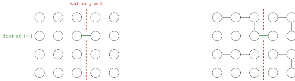
(a) The call links one pair and stops. Every other node is still isolated; no crossing was examined, let alone removed.
