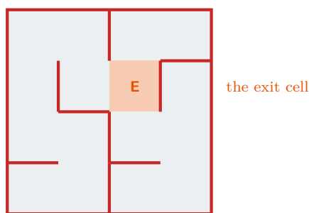
(a) The maze as walls. The area is enclosed; the exit is a cell, not a gap in the outer wall.
