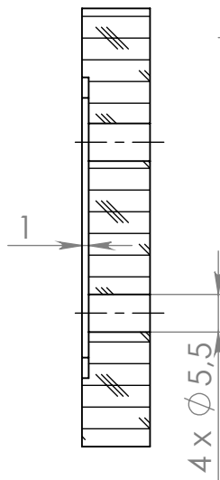
SECTION B-B SCALE 1 : 1
