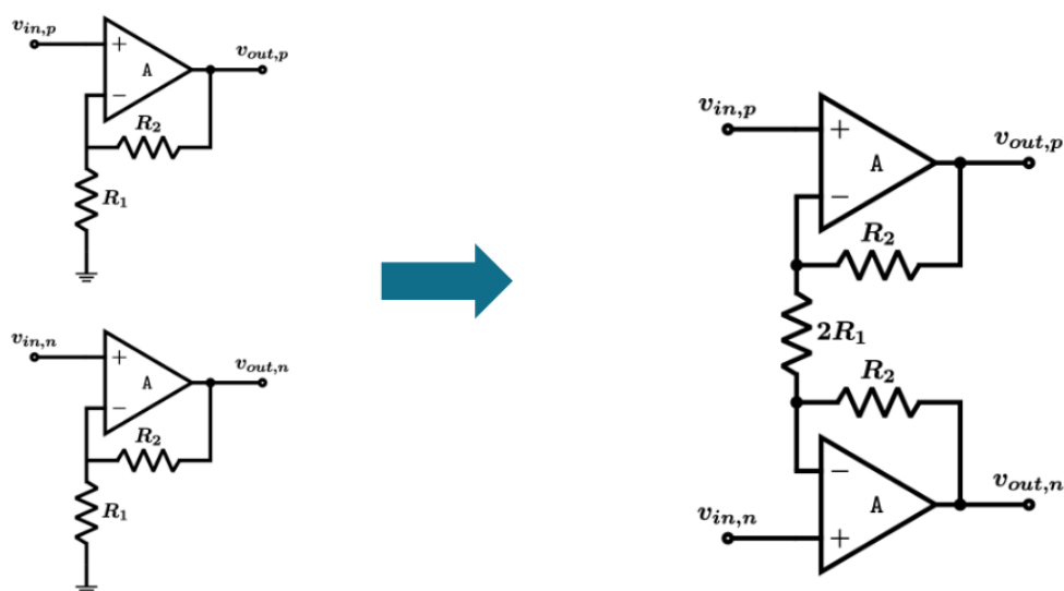
Figure 9: Instrumentation amplifier
