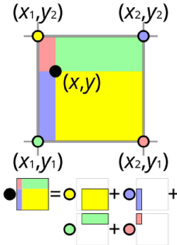
Figure 63: Bilinear interpolation (wikipedia)
