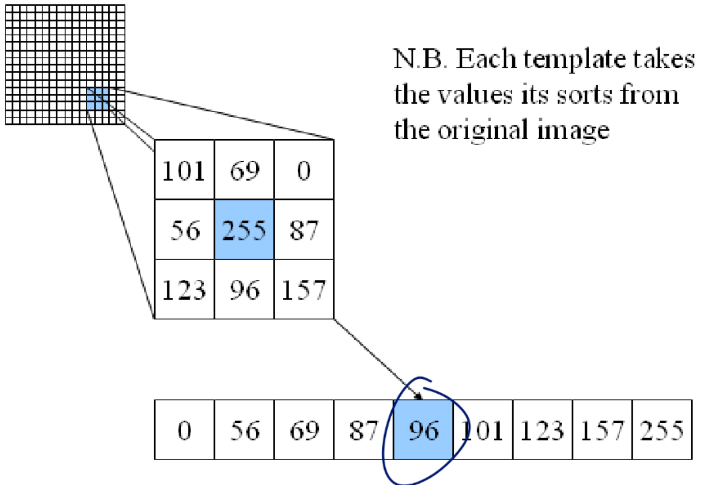
Figure 30: Median filters principle - credits: southampton.ac.uk
