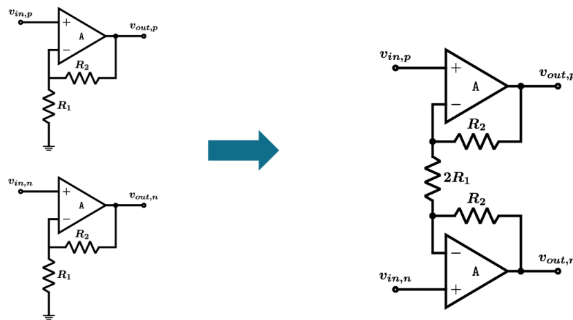
Figure 14: Instrumentation Amplifier
