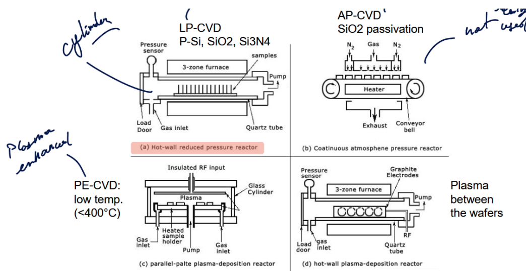
Figure 14: CVD Reactors
