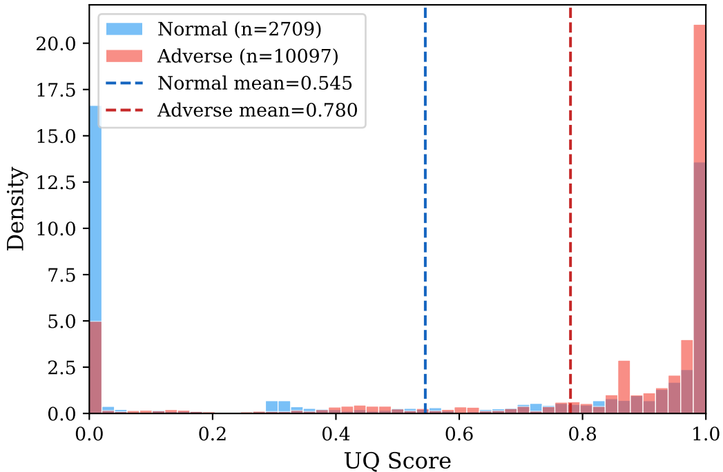
Uncertainty Score Distribution: Normal vs Adverse
