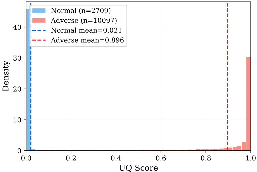
Uncertainty Score Distribution: Normal vs Adverse
