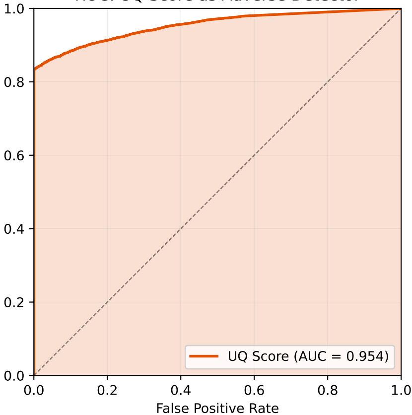
ROC: UQ Score as Adverse Detector
