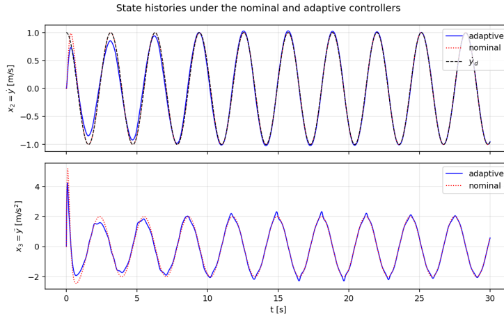
Figure 4: State histories x_2 = \dot{y} and x_3 = \ddot{y} under the nominal and adaptive controllers (the output x_1 = y is shown in Fig. 3).
