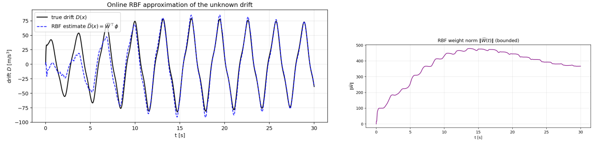
Figure 6: Online RBF approximation of the unknown drift D(\mathbf{x}) (left) and the bounded weight norm (right).
