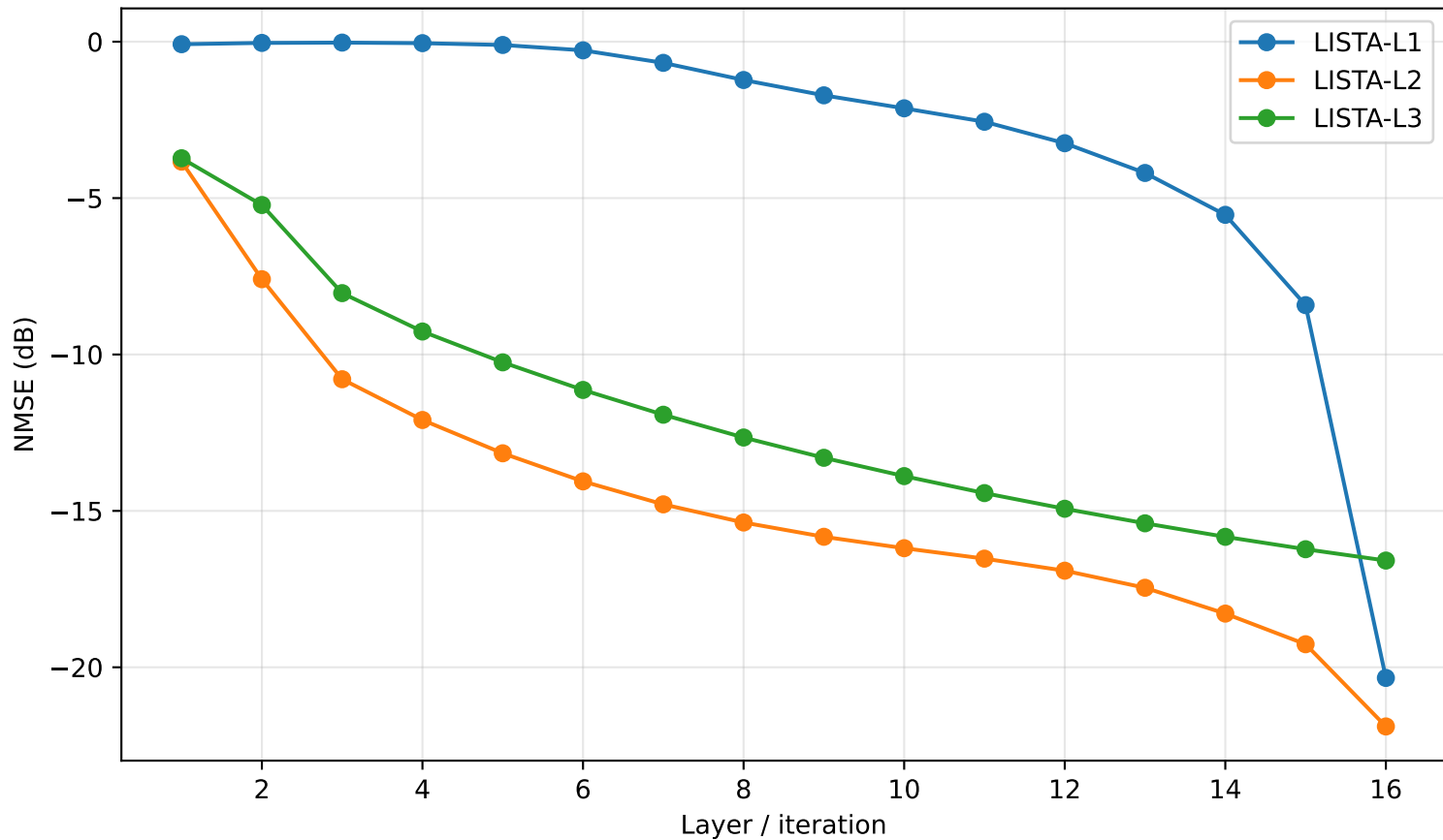
LISTA training methods: NMSE vs unfolded layer
