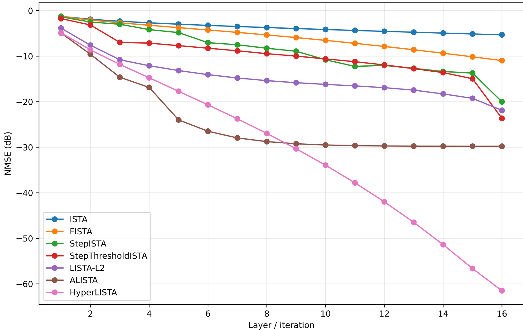
Main unfolded optimizers: NMSE vs layer
