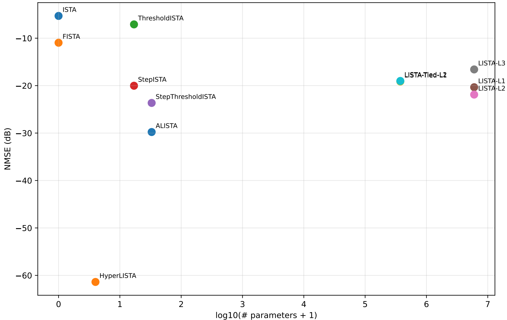
Accuracy-parameter tradeoff across ISTA-derived unfolded models
