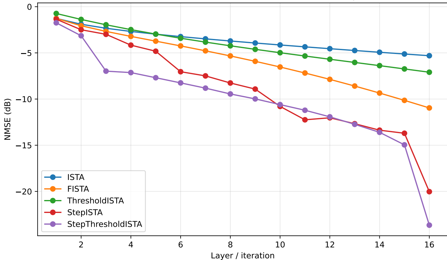
ISTA-derived scalar models: NMSE vs unfolded layer
