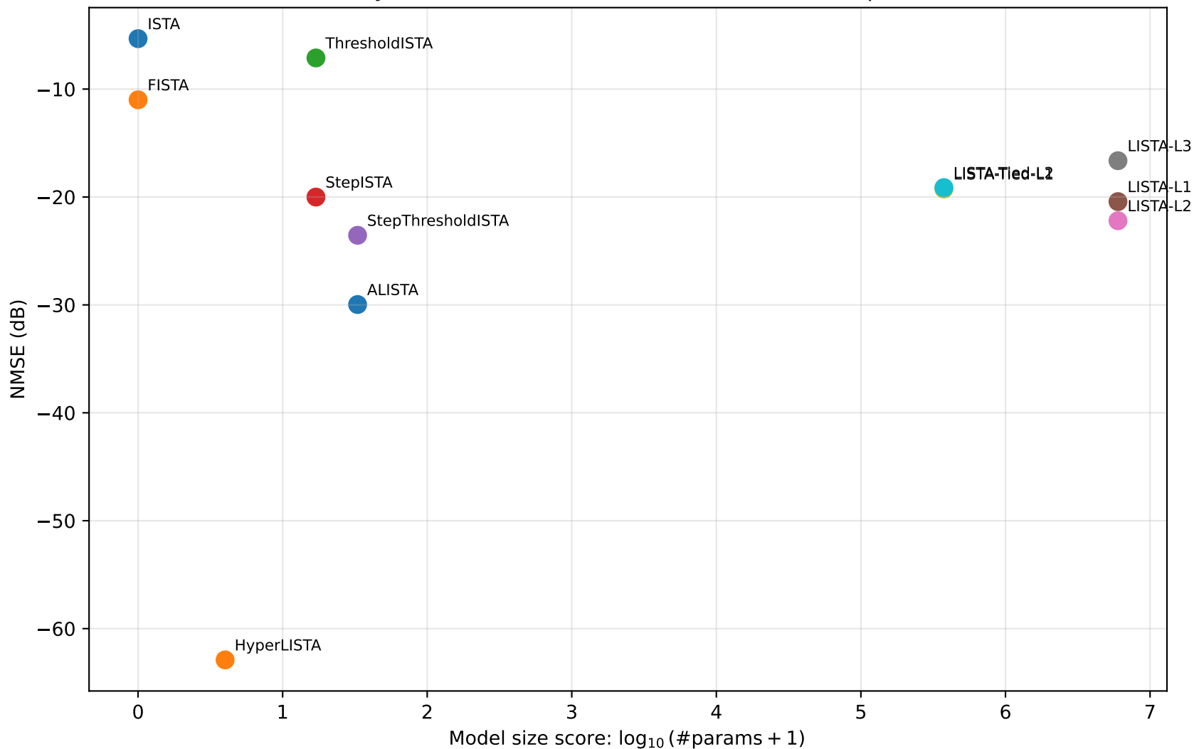
Accuracy vs model size for ISTA-derived unfolded optimizers
