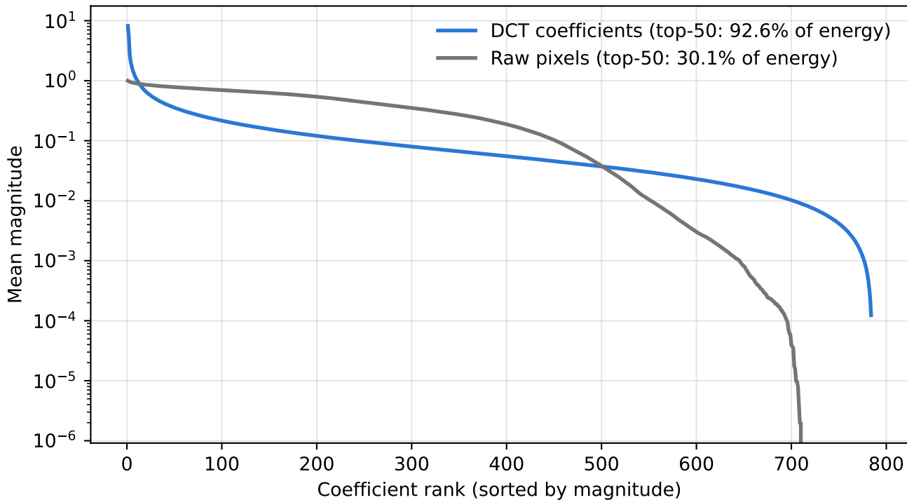
FASHIONMNIST: DCT coefficients decay, pixels do not
