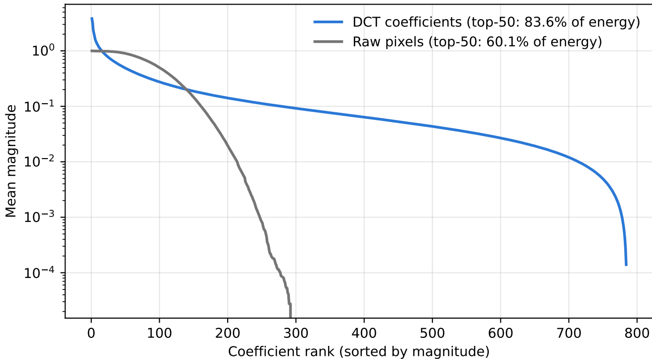
MNIST: DCT coefficients decay, pixels do not
