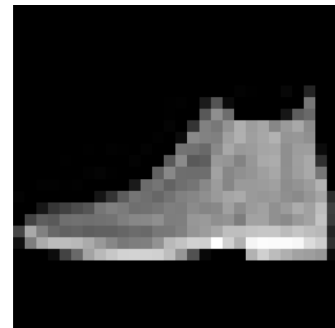
Original
