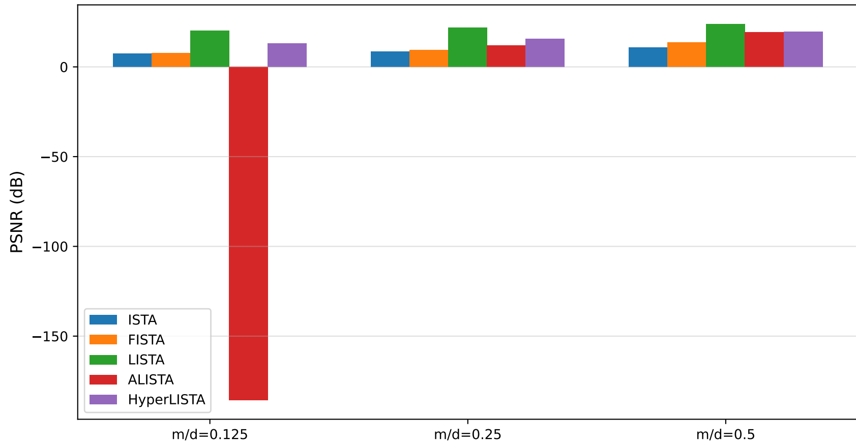
PSNR vs. Measurement Ratio — Fashion-MNIST CS
