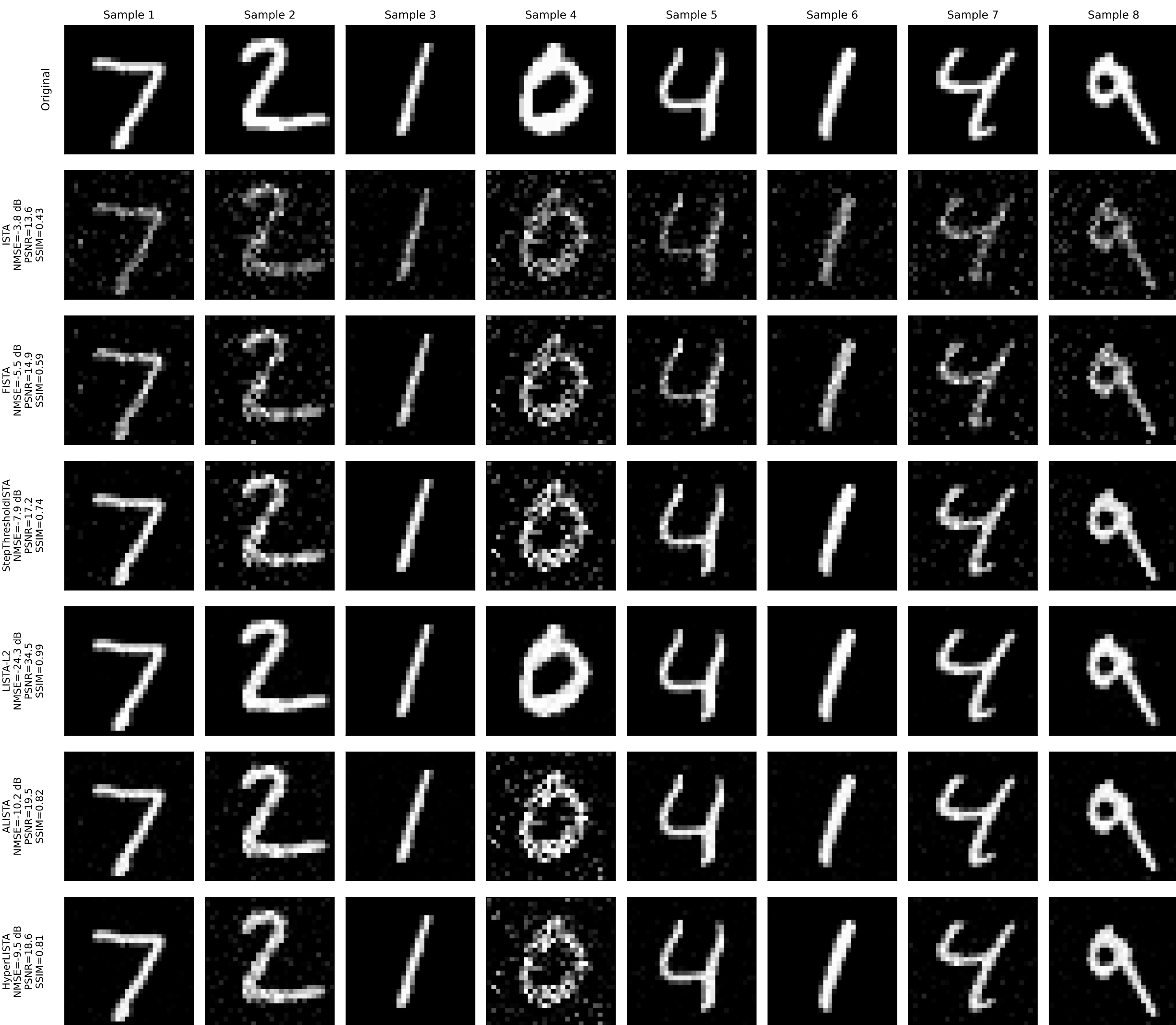
MNIST Pixel-Domain Compressed Sensing Reconstructions
