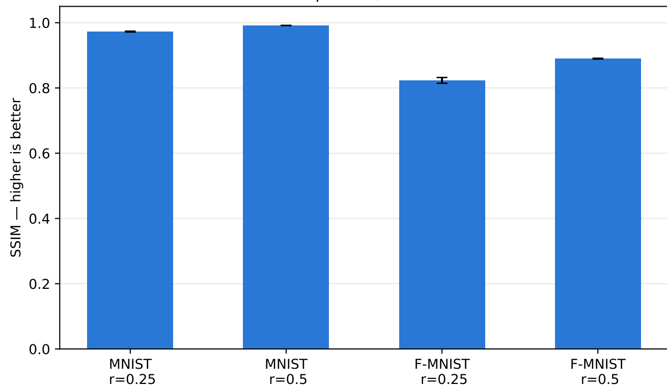
Part B: LISTA-L2 SSIM per cell, mean \pm std over 3 seeds
