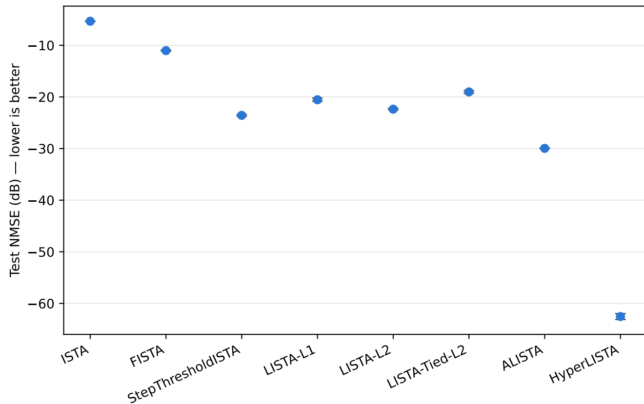
Part A: mean \pm std over 5 seeds
