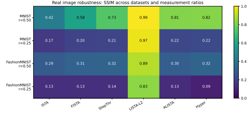
Figure 4: Robustness sweep (Part B): SSIM across \{\text{MNIST}, \text{Fashion-MNIST}\} \times \text{ratio} \{0.25, 0.5\} . LISTA-L2 stays high in all four scenarios; the Gaussian-sparse-prior methods degrade sharply with data complexity and measurement scarcity.
