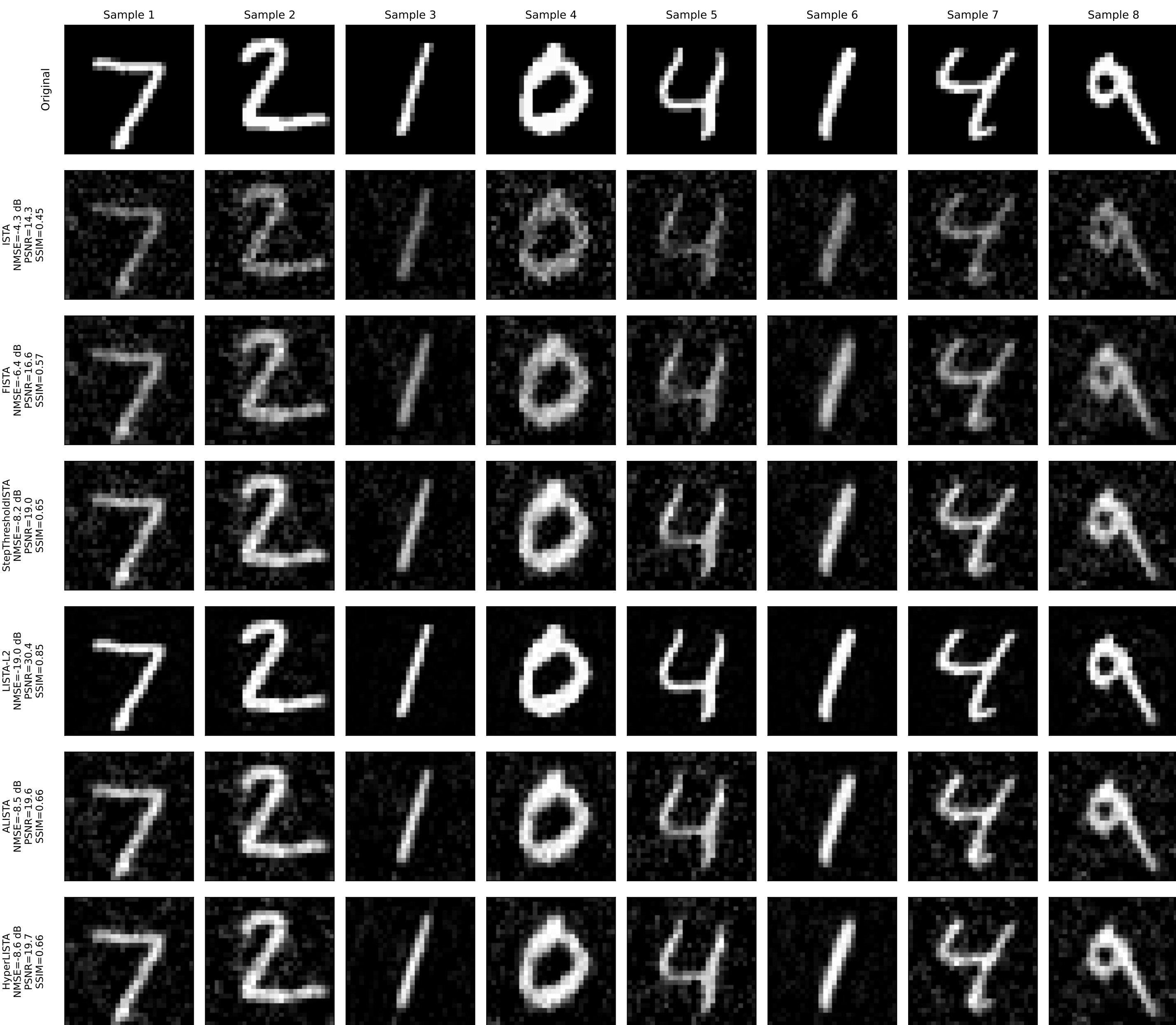
MNIST DCT-Domain Compressed Sensing Reconstructions
