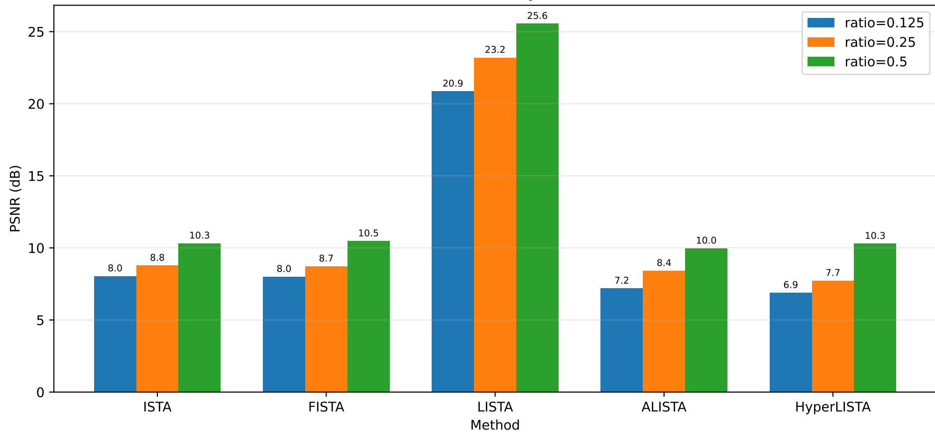
Fashion-MNIST Pixel-Domain CS — PSNR by Method and Measurement Ratio
