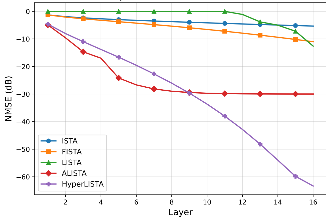
NMSE vs. Layer ( m=250 , n=500 , s=50 , noiseless)
