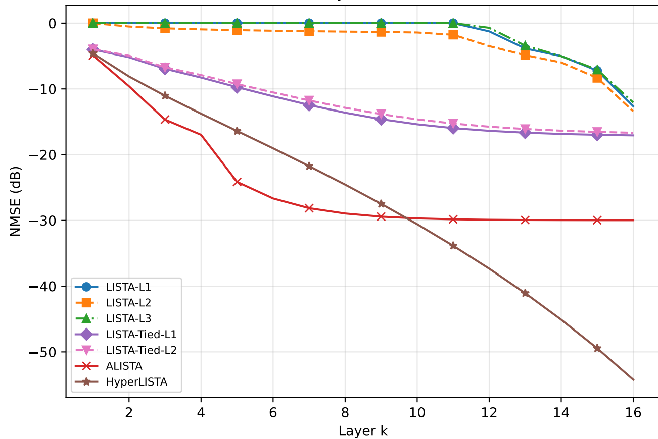
NMSE vs Layer — All Methods
