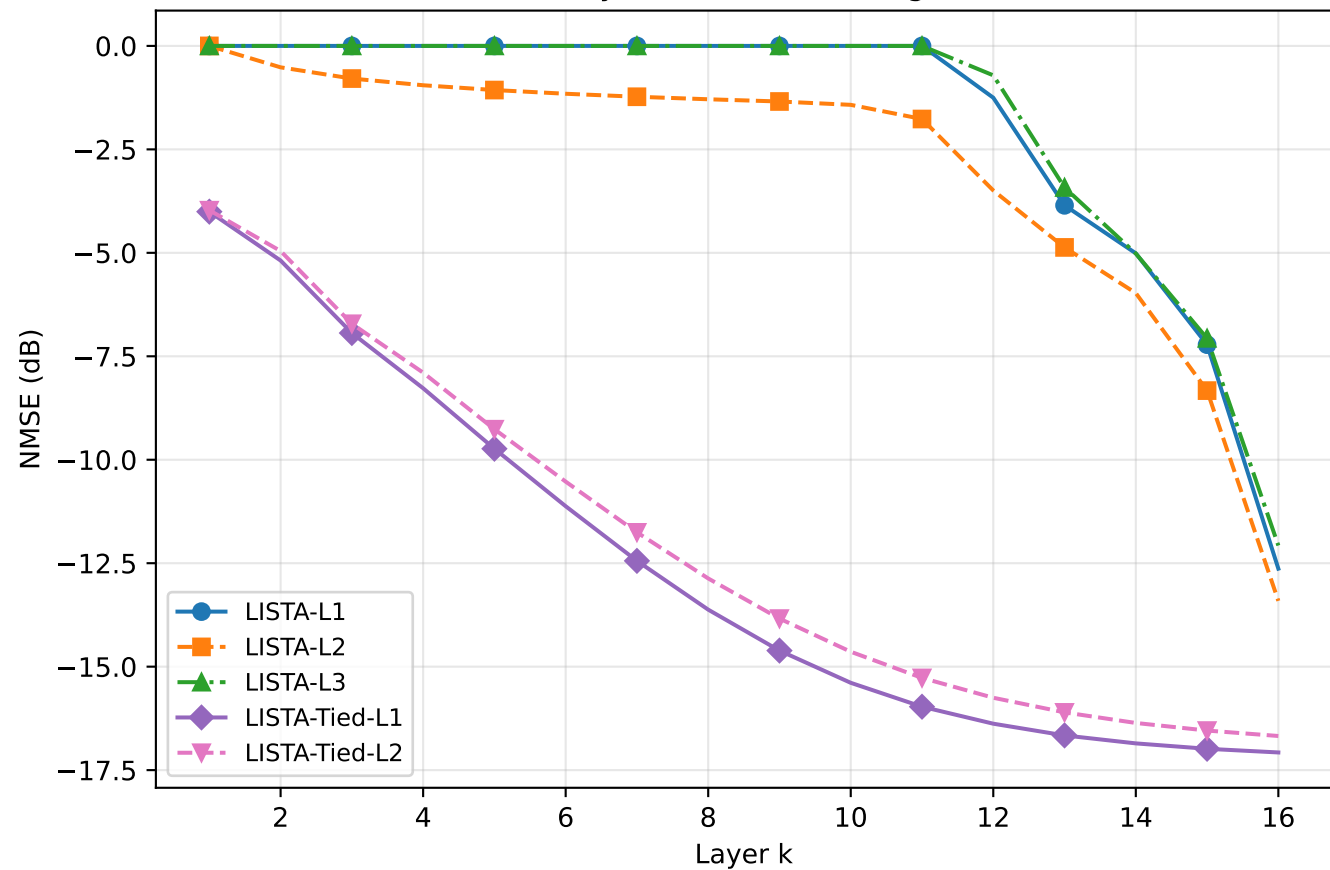
NMSE vs Layer — LISTA Training Methods
