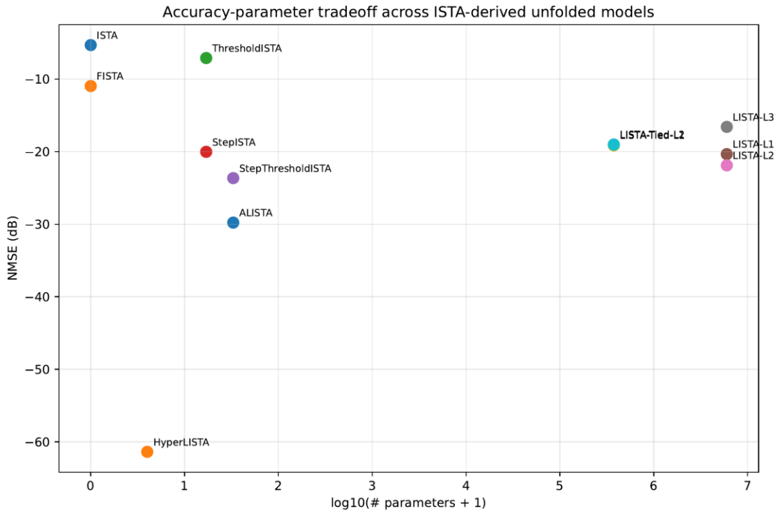
Figure 2. Accuracy versus parameter count. The scalar models occupy the useful low-parameter region.
