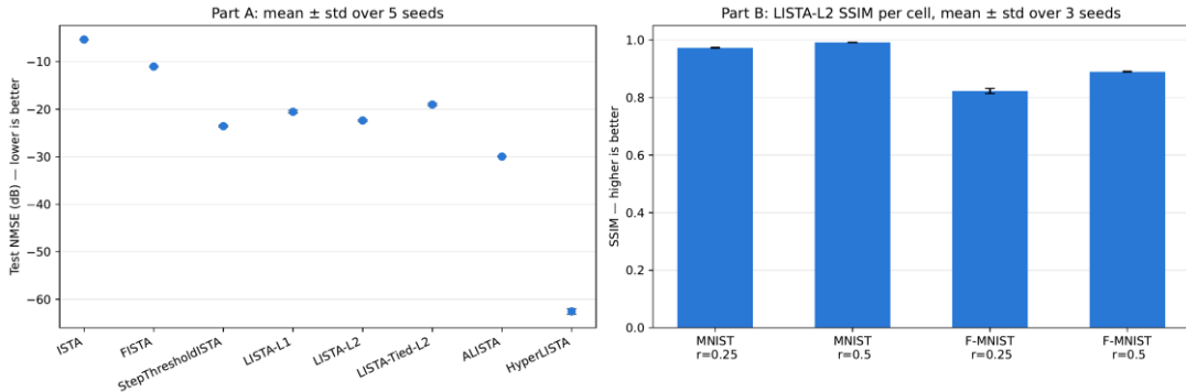
Figure 5. Multi-seed results for synthetic NMSE across models (left) and pixel-domain LISTA-L2 SSIM across datasets and measurement ratios (right).
