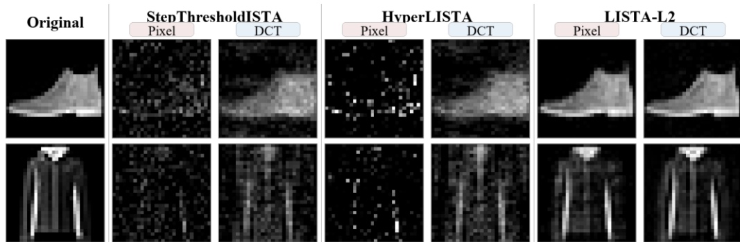
Figure 4. Representative Fashion-MNIST reconstructions at measurement ratio 0.25 using the same measurements. StepThresholdISTA and HyperLISTA largely collapse in the pixel domain but recover recognizable structure with DCT, while LISTA-L2 remains strong in both representations.
