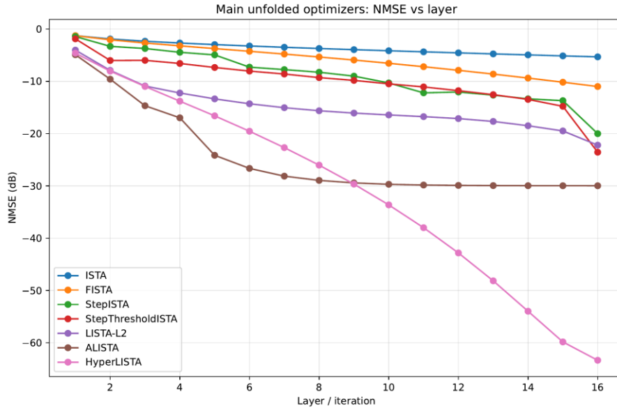
Figure 1. NMSE across the 16 unfolded layers for the main synthetic models.
