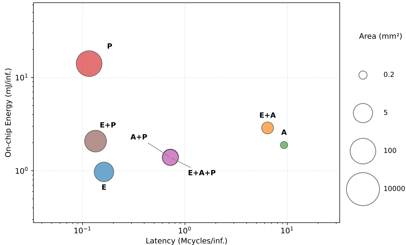
Configurations against Eyeriss v2: MobileNet V1 INT8
