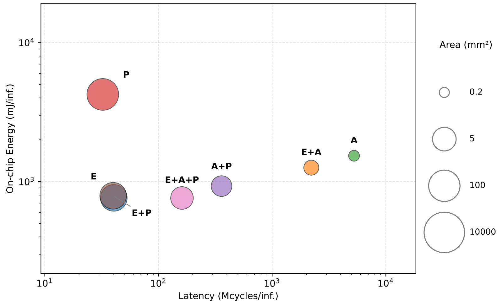
Configurations against SAURIA: VGG-16 FP16
