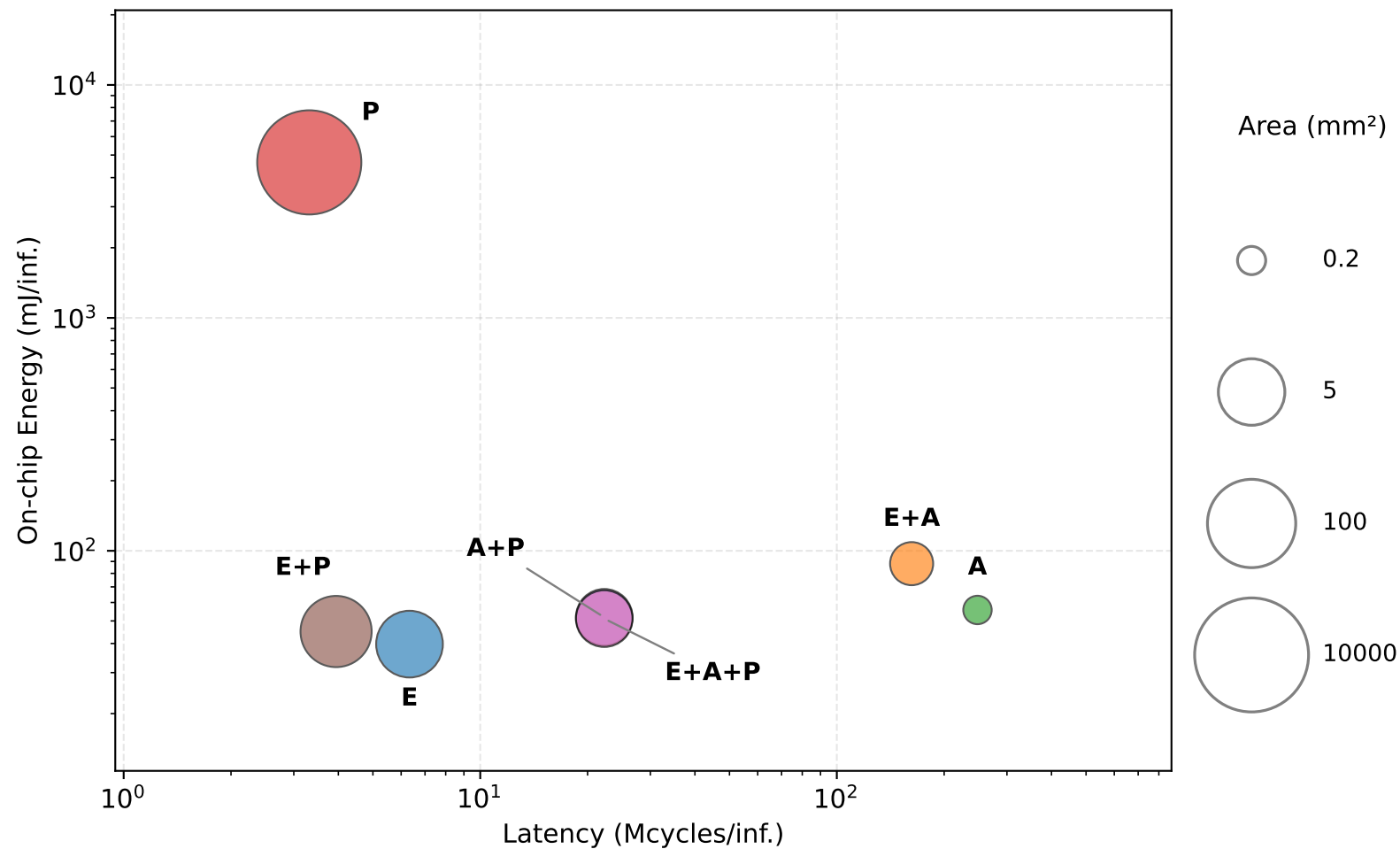
End-to-End INT16 AlexNet configurations
