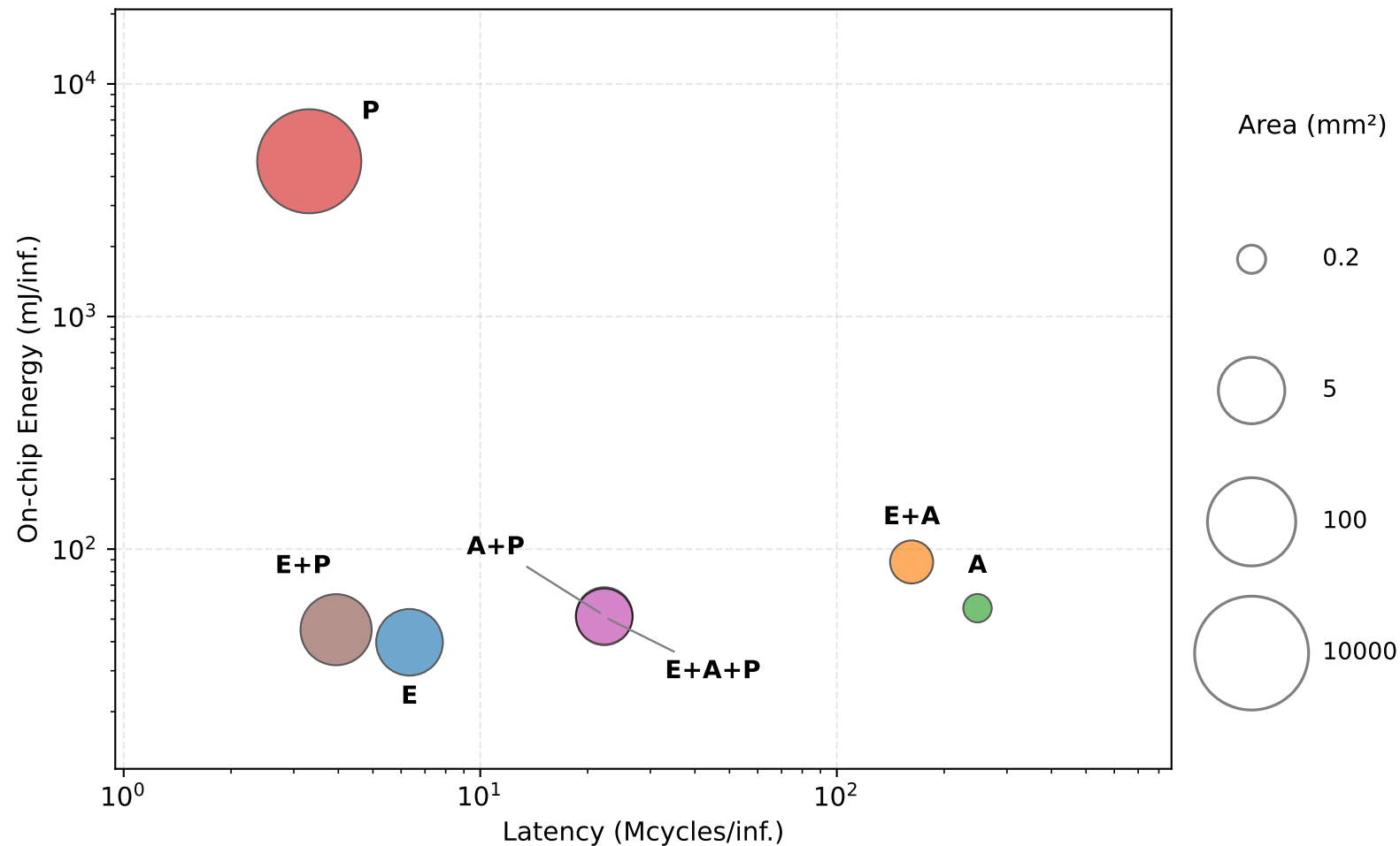
Talos — AlexNet INT16
