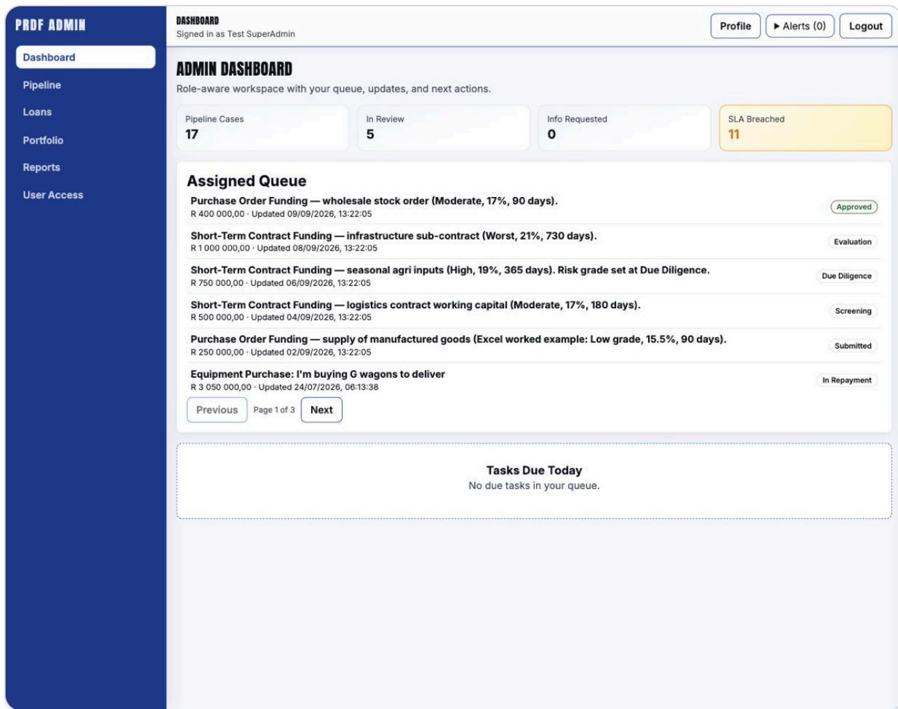
Figure 3 — Admin dashboard
