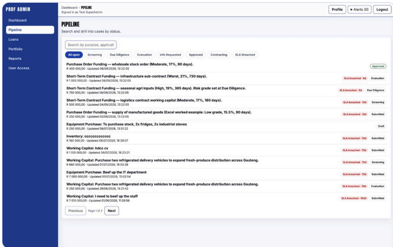
Figure 4 — Pipeline list
