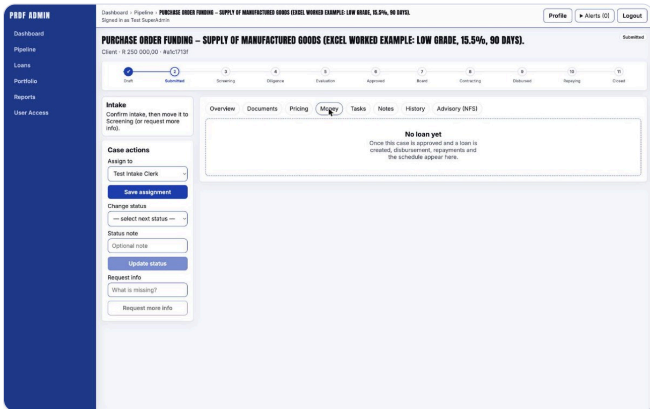
Figure 8 — Money tab
