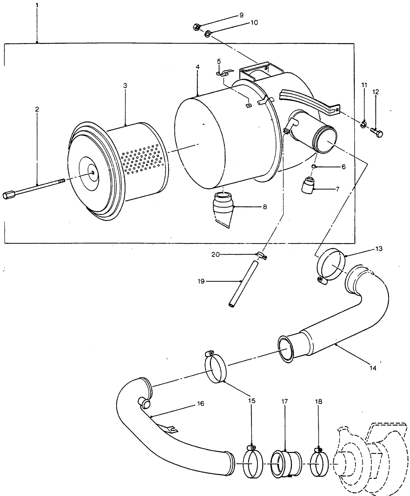
AIR CLEANER ASSEMBLY, INTAKE AND CONNECTIONS
