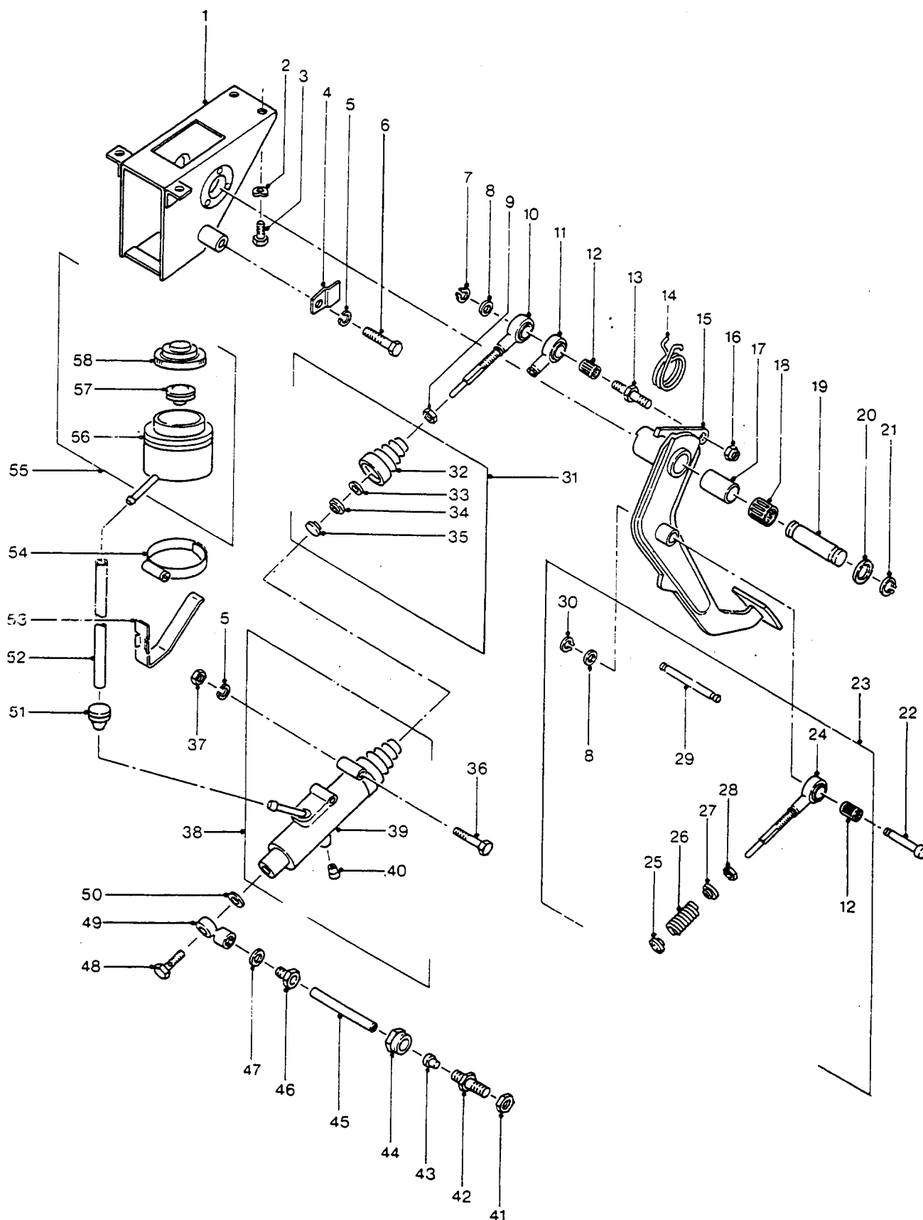
CLUTCH MASTER CYLINDER, PEDAL AND BRACKET
