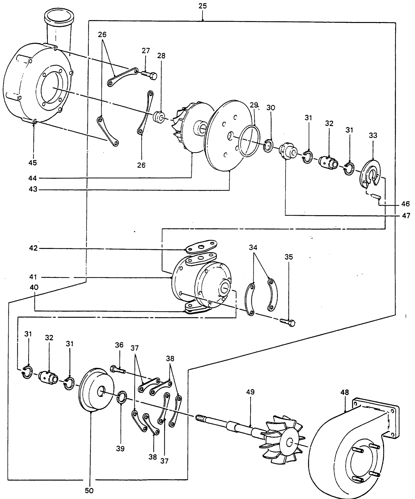
TURBOCHARGER, AIRESEARCH
