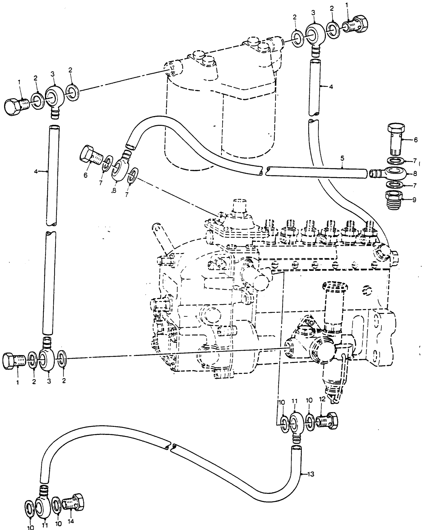
FUEL PUMP, LINES AND CONNECTIONS
