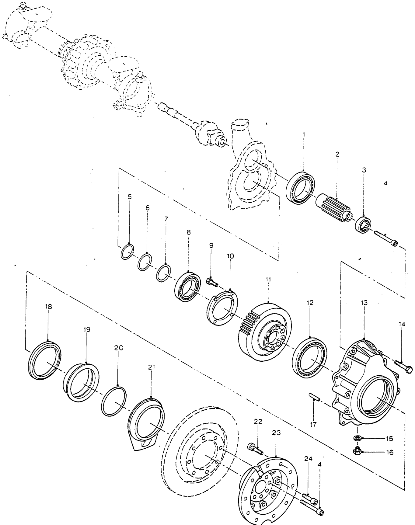
WHEEL HUB DRIVES, FRONT AXLE
