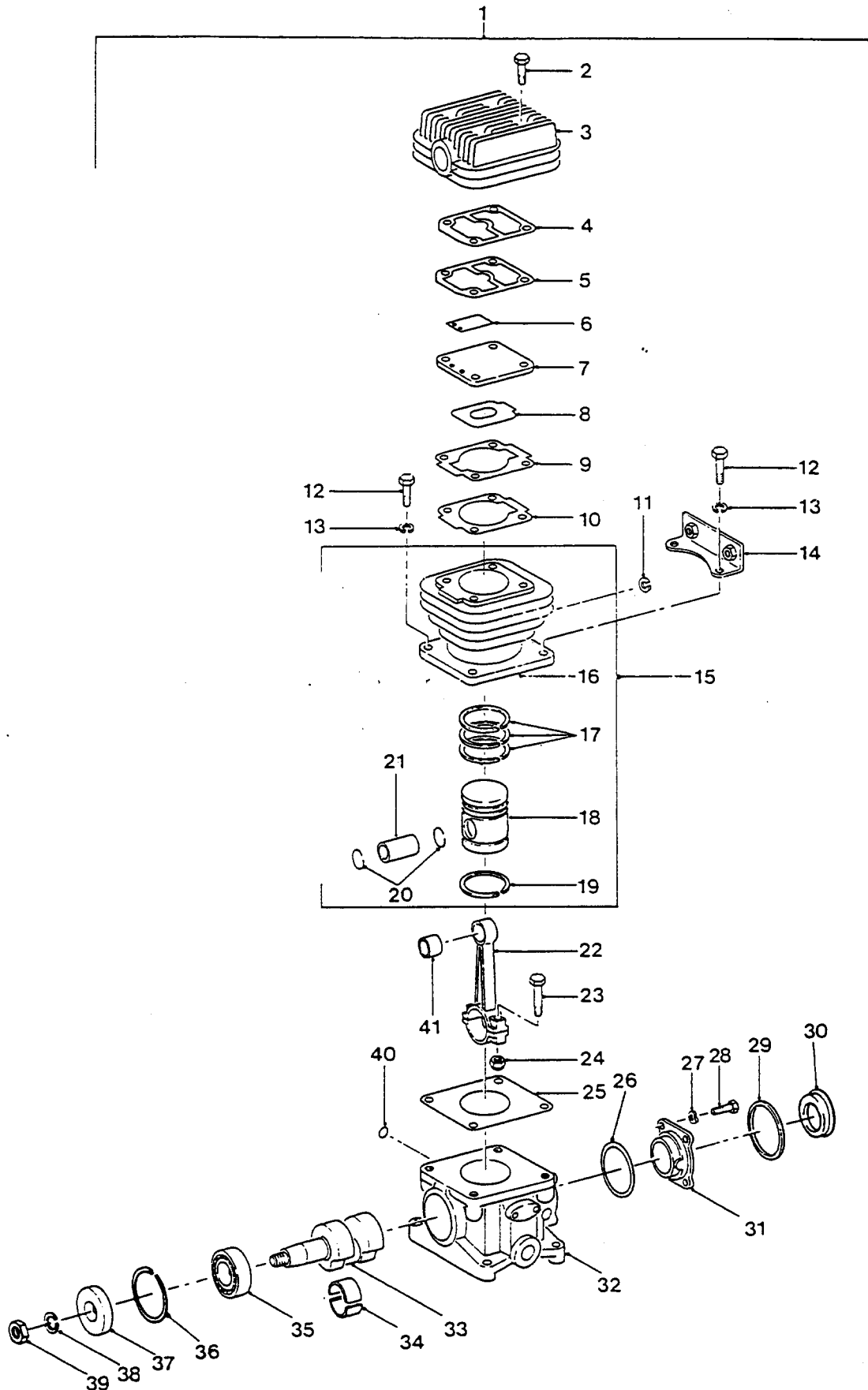
AIR COMPRESSOR, DRIVE BELT, PIPING AND MOUNTS
