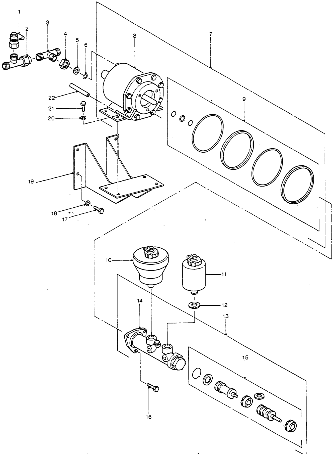
DUAL CIRCUIT MASTER CYLINDER
