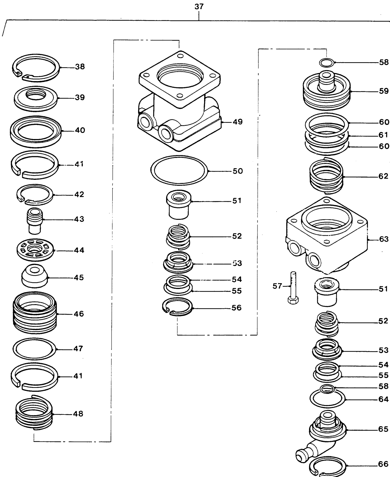
BRAKE TREADLE VALVE, DUAL CIRCUIT (WABCO)
